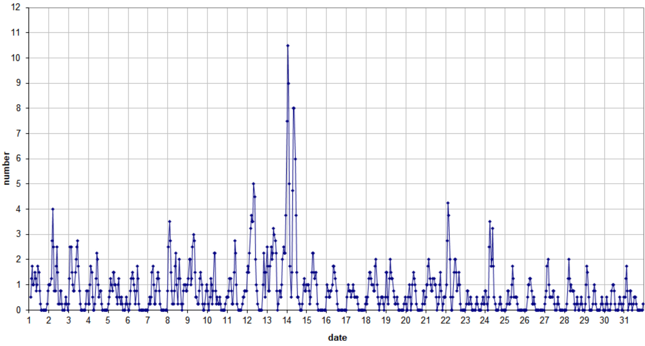
49.99MHz - RadioMeteors December 2024 number of reflections >10 seconds per hour (weighted average) Felix Verbelen (Kamphenhout)
