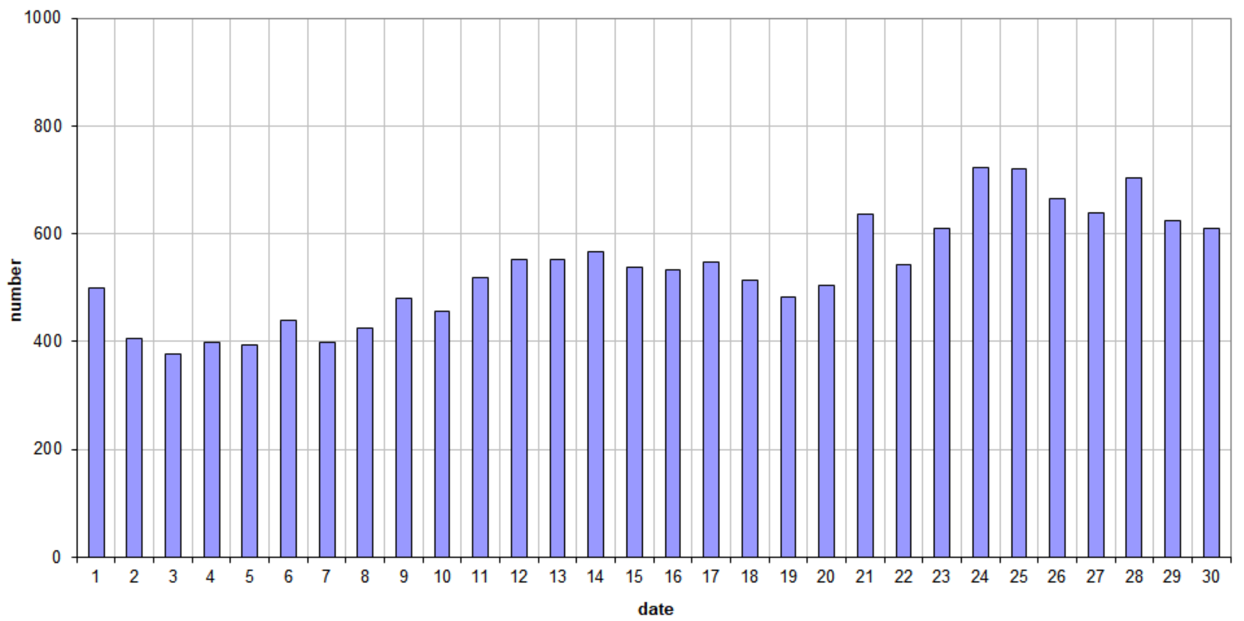
49.99MHz - RadioMeteors April 2025 daily totals of "all" reflections (automatic count_Mettel5_7Hz) Felix Verbelen (Kamphenhout)
