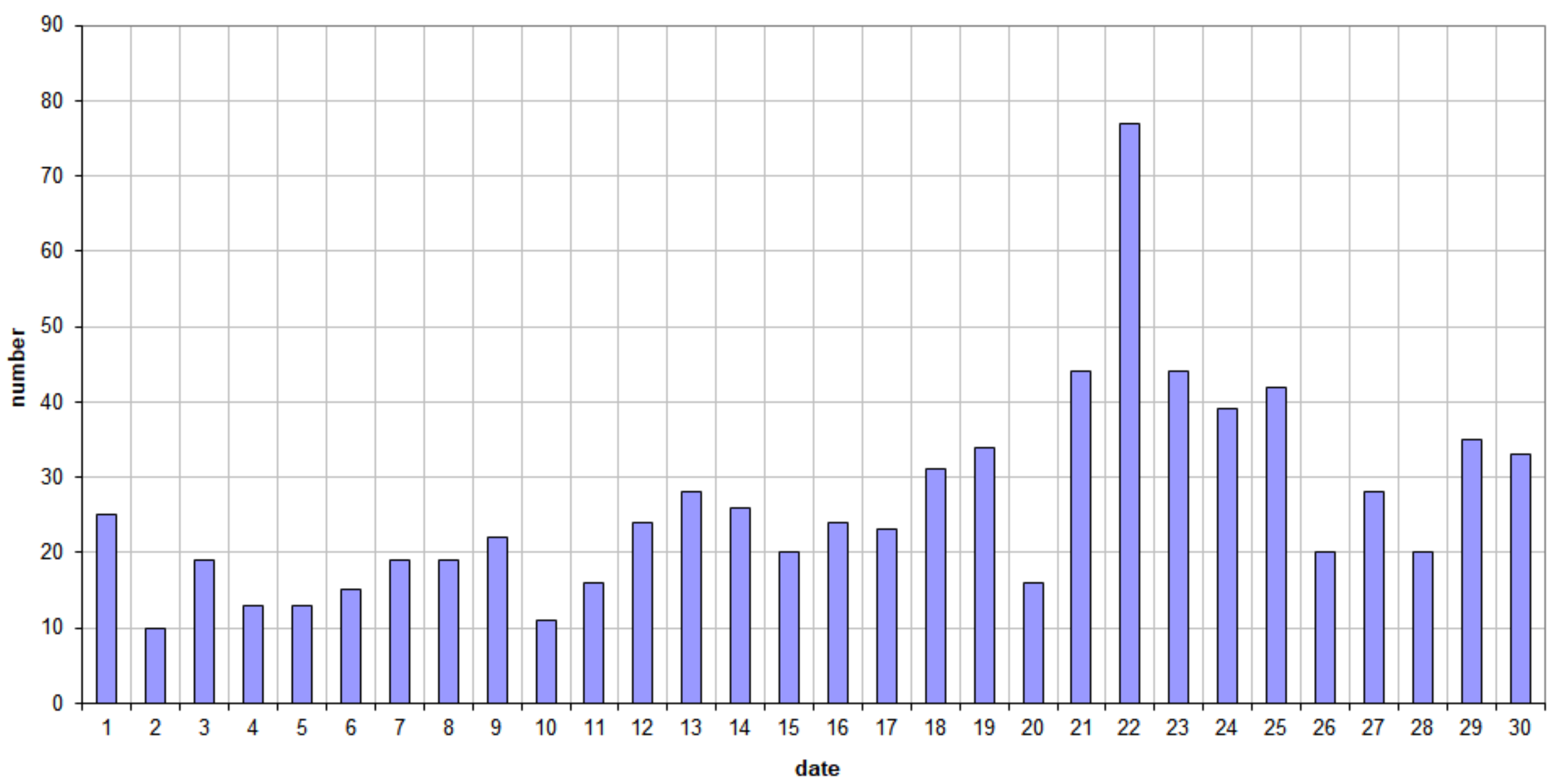
49.99MHz - RadioMeteors April 2025 daily totals of all overdense reflections Felix Verbelen (Kamphenhout)
