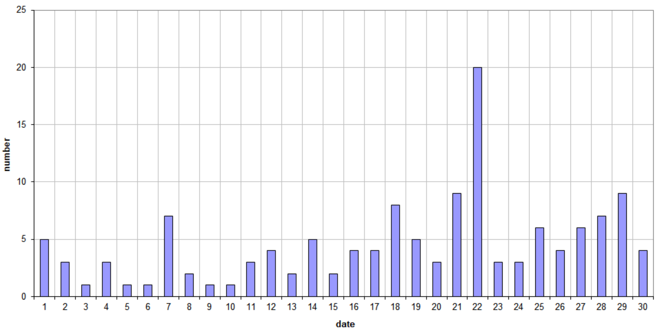
49.99MHz - RadioMeteors April 2025 daily totals of reflections longer than 10 seconds Felix Verbelen (Kamphenhout)
