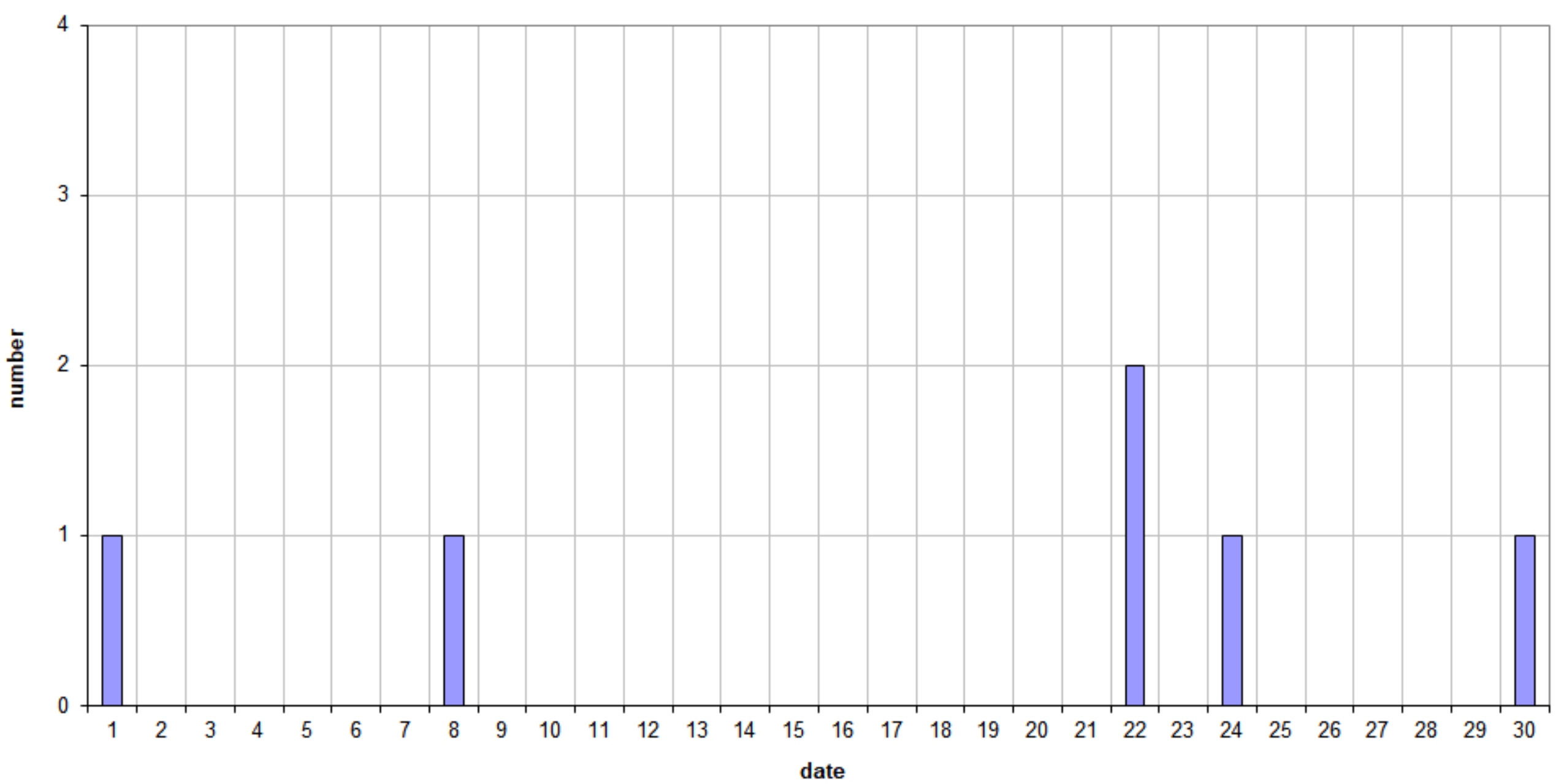
49.99MHz - RadioMeteors April 2025 daily totals of reflections longer than 1 minute Felix Verbelen (Kamphenhout)
