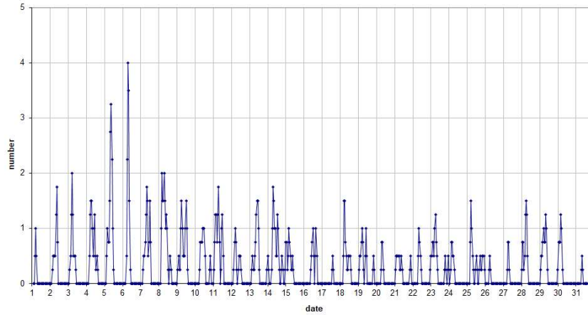
49.99MHz - RadioMeteors May 2025 number of reflections >10 seconds per hour (weighted average) Felix Verbelen (Kamphenhout)
