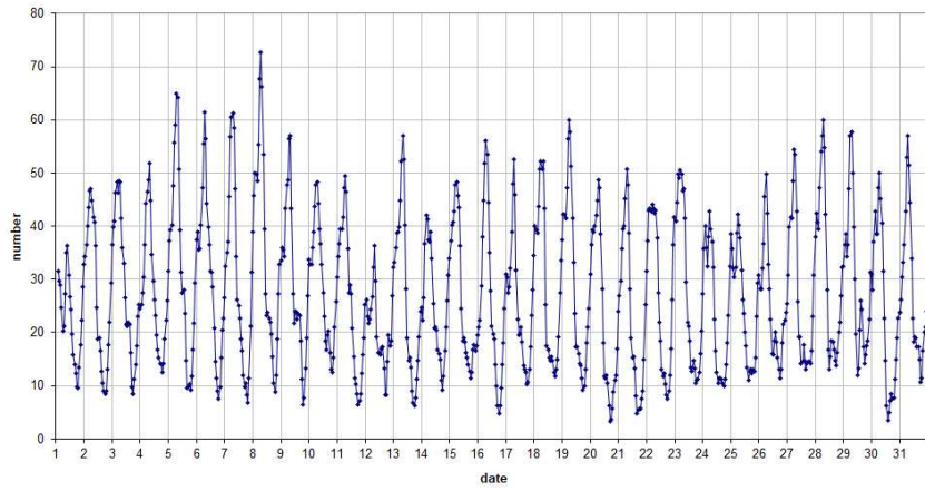
49.99 MHz - RadioMeteors May 2025 number of "all" reflections per hour (weighted average) (automatic count_Mette15_THz) Felix Verbelen (Kamphenhout)
