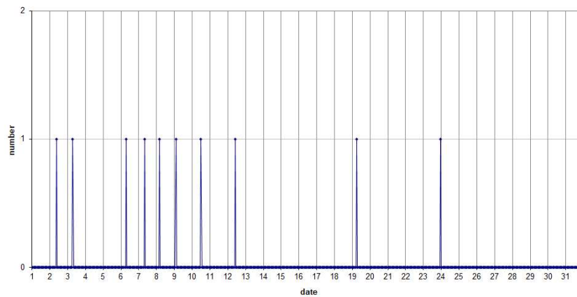
49.99MHz - RadioMeteors May 2025 hourly totals of overdense reflections longer than 1 minute Felix Verbelen (Kamphenhout/BE)
