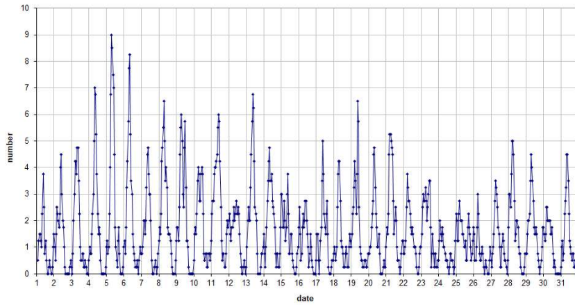
49.99MHz - RadioMeteors May 2025 number of overdense reflections per hour (weighted average) Felix Verbelen (Kamphenhout)
