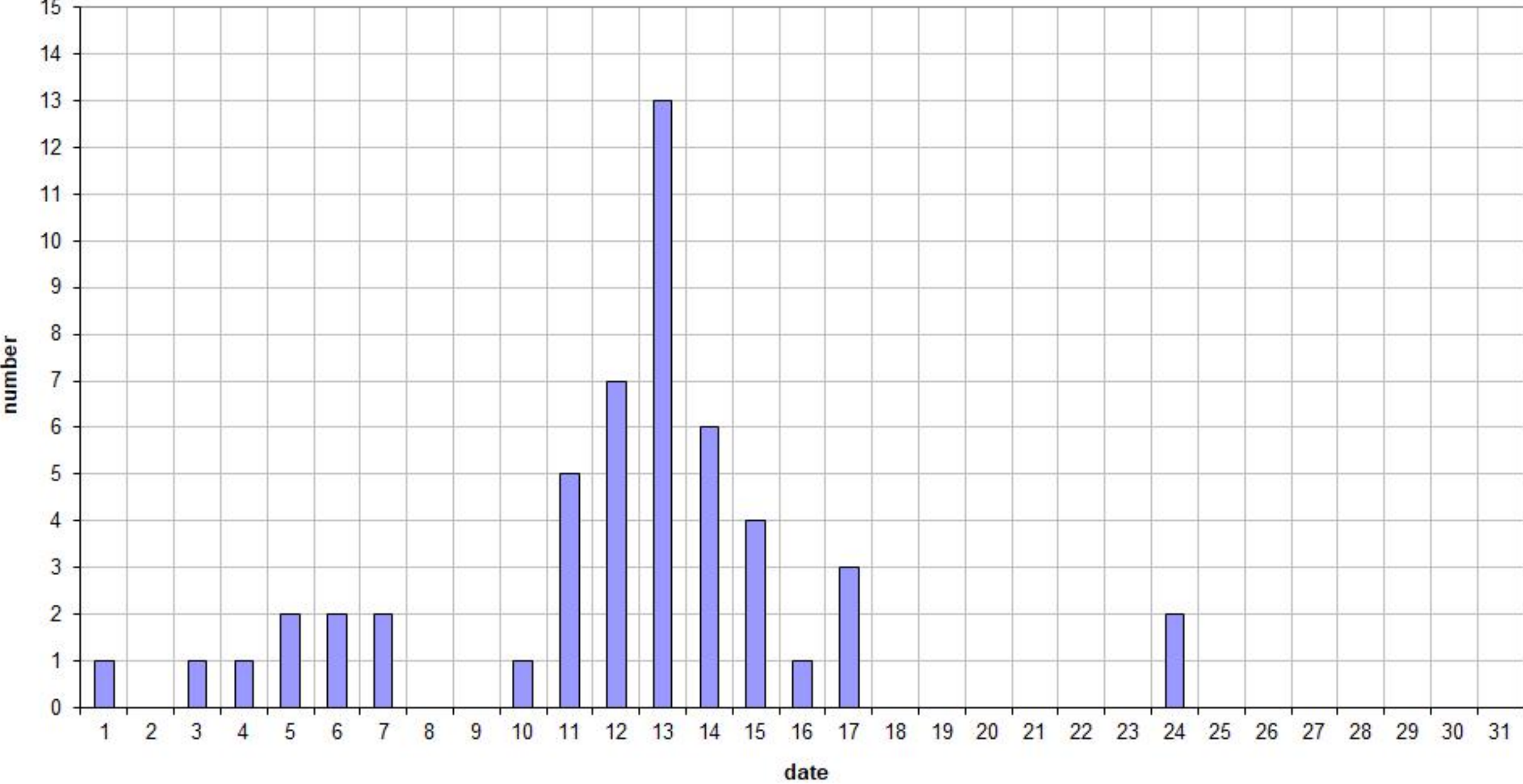
49.99MHz - RadioMeteors August 2025 daily totals of reflections longer than 1 minute Felix Verbelen (Kamphenhout)
