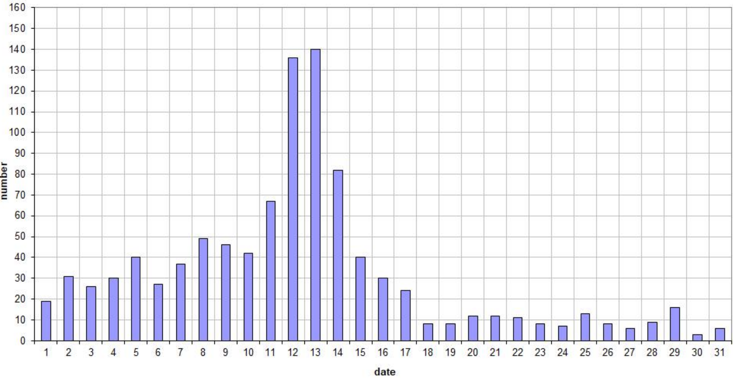
49.99MHz - RadioMeteors August 2025 daily totals of reflections longer than 10 seconds Felix Verbelen (Kamphenhout)
