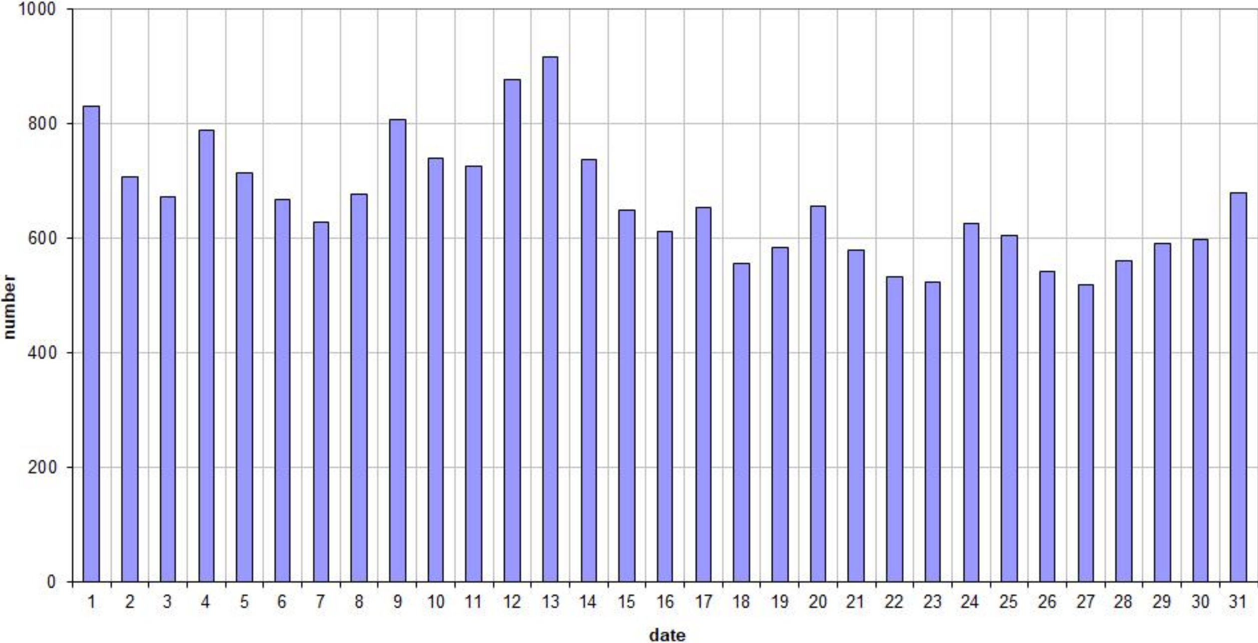
49.99MHz - RadioMeteors August 2025 daily totals of "all" reflections (automatic count_Mettel5_7Hz) Felix Verbelen (Kamphenhout)
