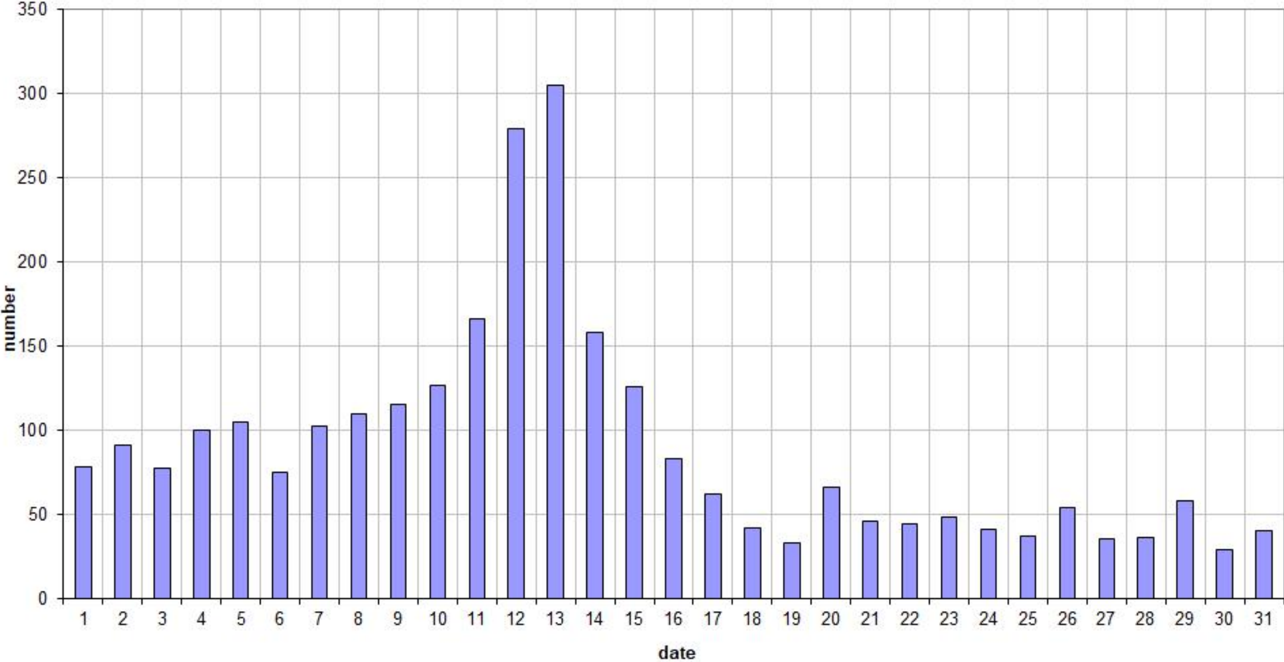
49.99MHz - RadioMeteors August 2025 daily totals of all overdense reflections Felix Verbelen (Kamphenhout)
