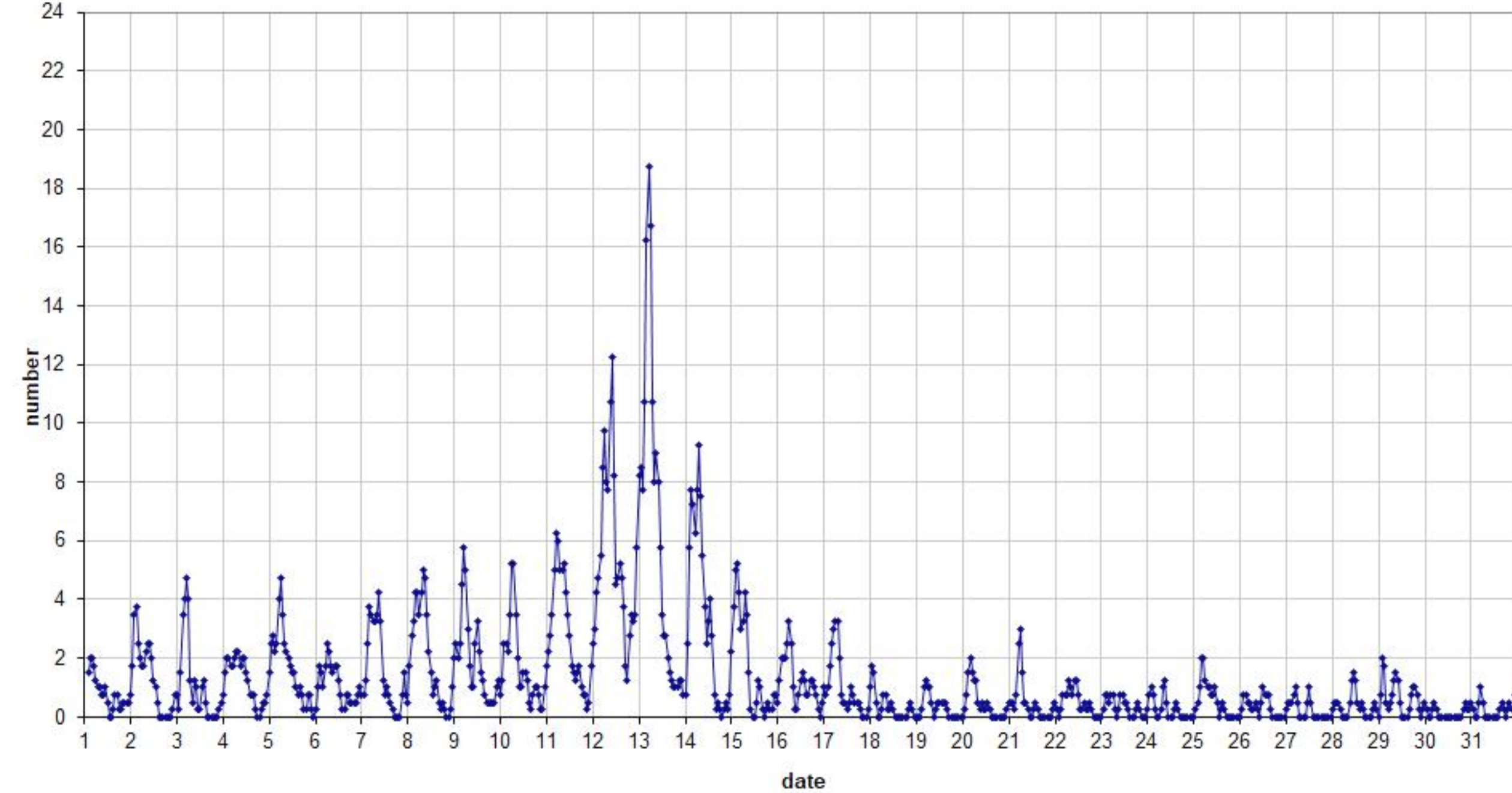
49.99MHz - RadioMeteors August 2025 number of reflections >10 seconds per hour (weighted average) Felix Verbelen (Kampenhout)
