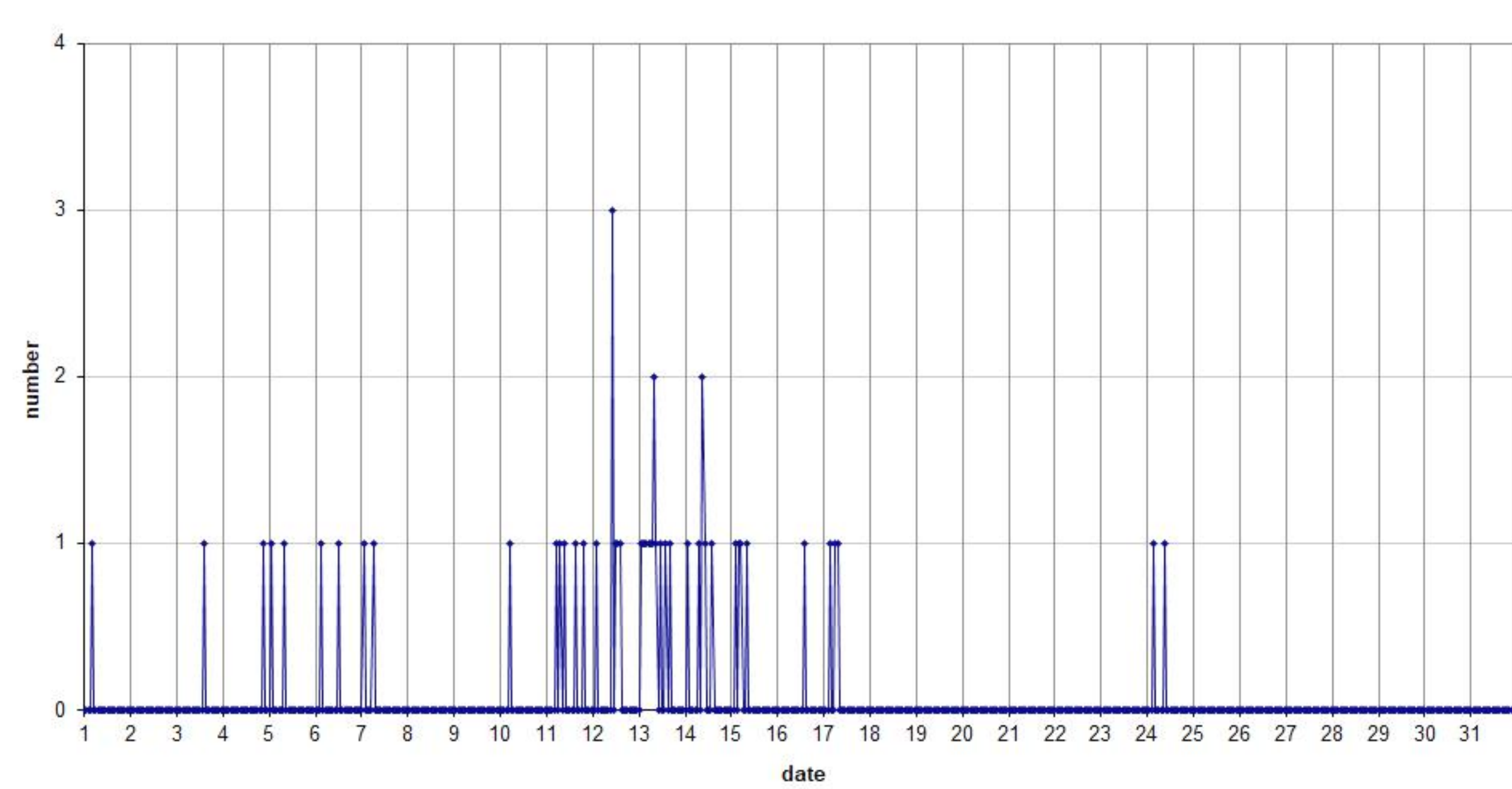
49.99MHz - RadioMeteors August 2025 hourly totals of overdense reflections longer than 1 minute Felix Verbelen (Kampenhout/BE)
