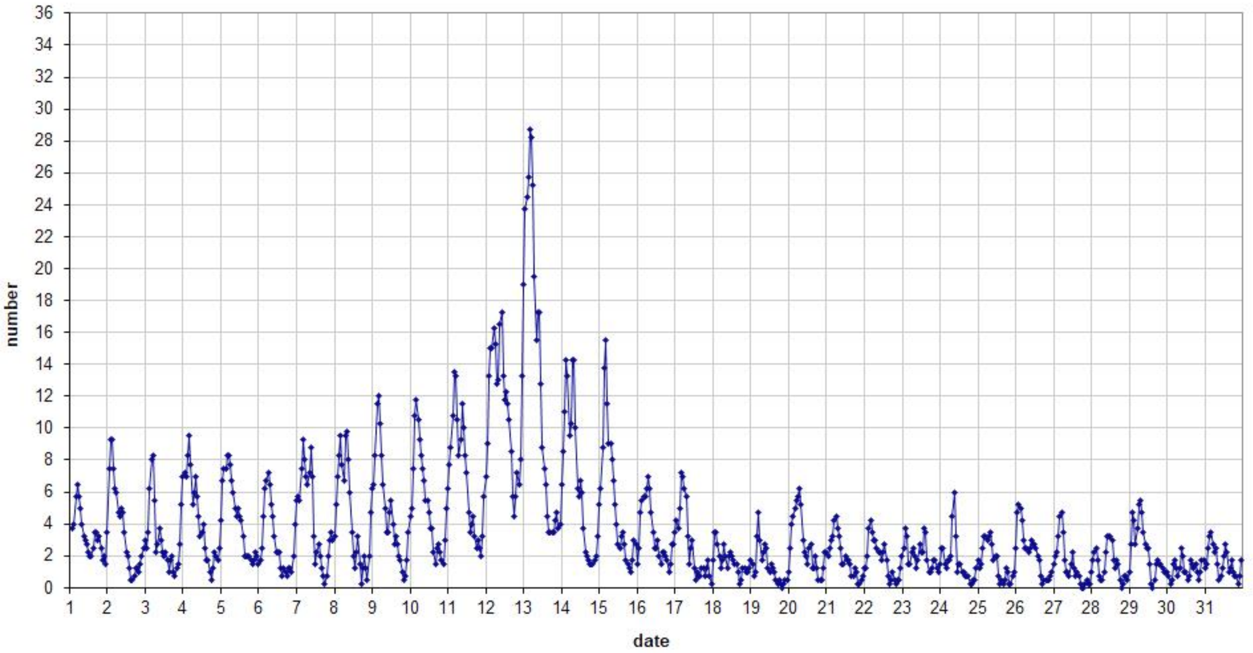
49.99MHz - RadioMeteors August 2025 number of overdense reflections per hour (weighted average) Felix Verbelen (Kampenhout)
