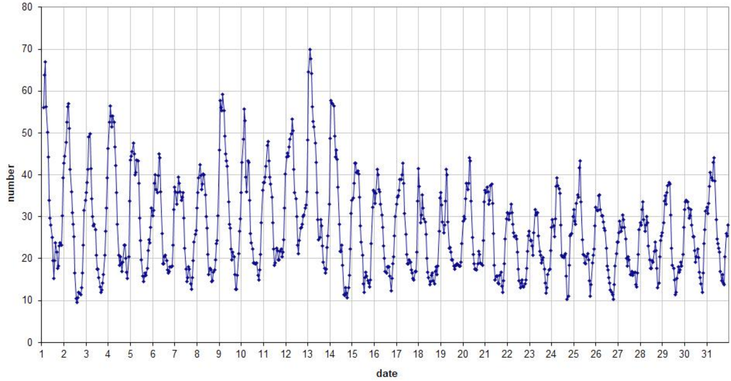
49.99 MHz - RadioMeteors August 2025 number of "all" refections per hour (weighted average) (automatic count_Mettel5_7Hz) Felix Verbelen (Kampenhout)
