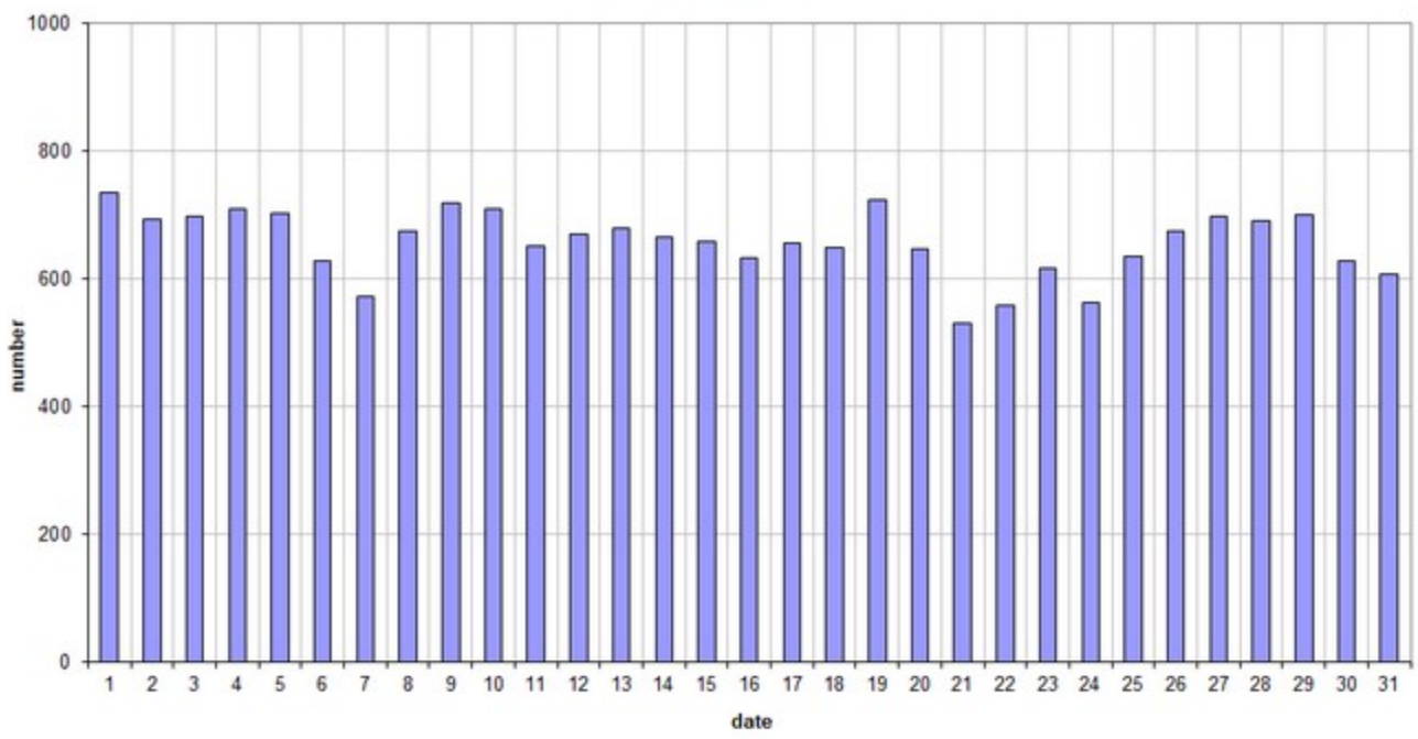
49.99MHz - RadioMeteors October 2025 daily totals of "all" reflections (automatic count_Mettel5_7Hz) Felix Verbelen (Kamphenhout)
