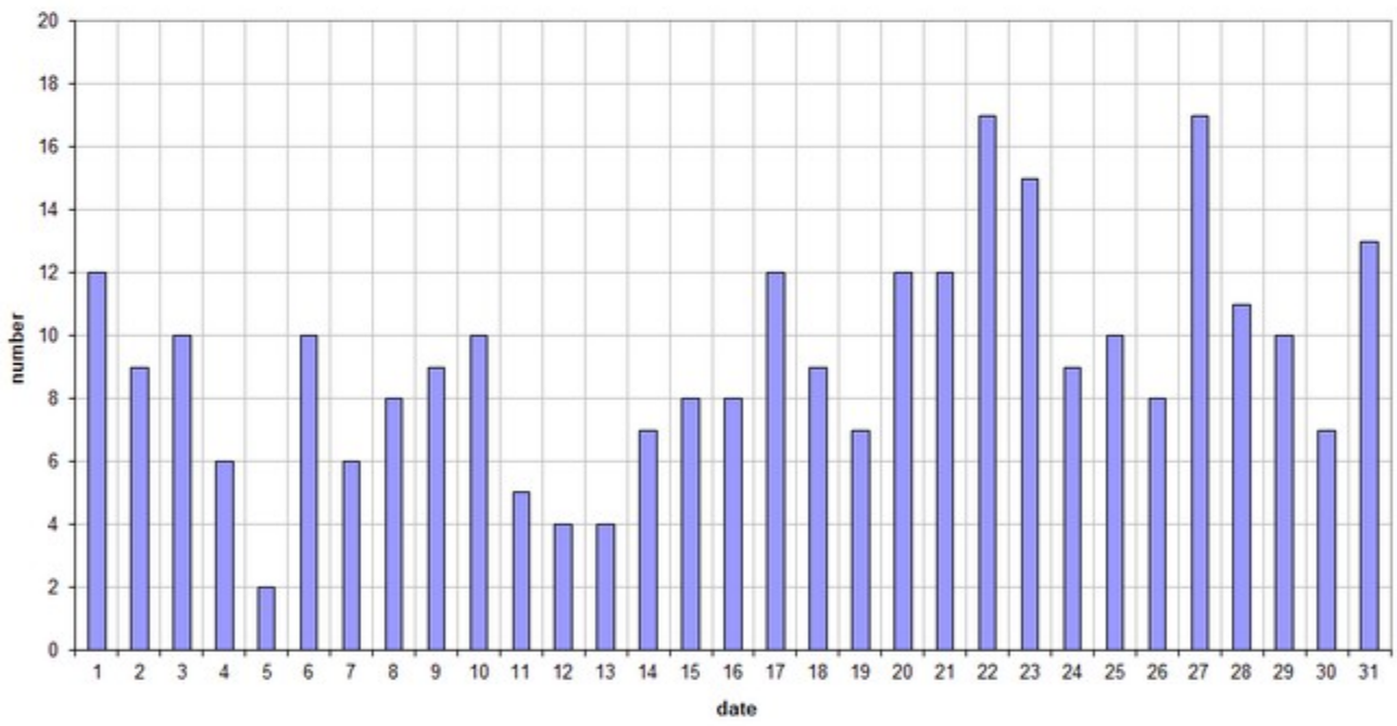
49.99MHz - RadioMeteors October 2025 daily totals of reflections longer than 10 seconds Felix Verbelen (Kamphenhout)
