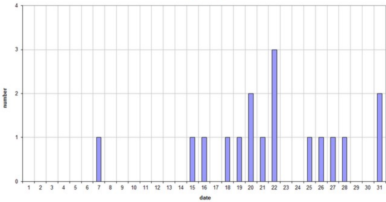
49.99MHz - RadioMeteors October 2025 daily totals of reflections longer than 1 minute Felix Verbelen (Kamphenhout)
