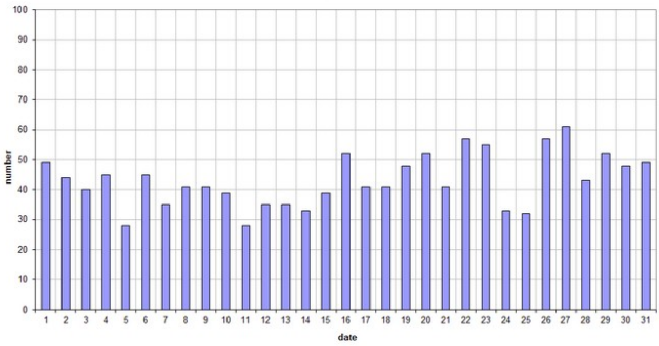
49.99MHz - RadioMeteors October 2025 daily totals of all overdense reflections Felix Verbelen (Kamphenhout)
