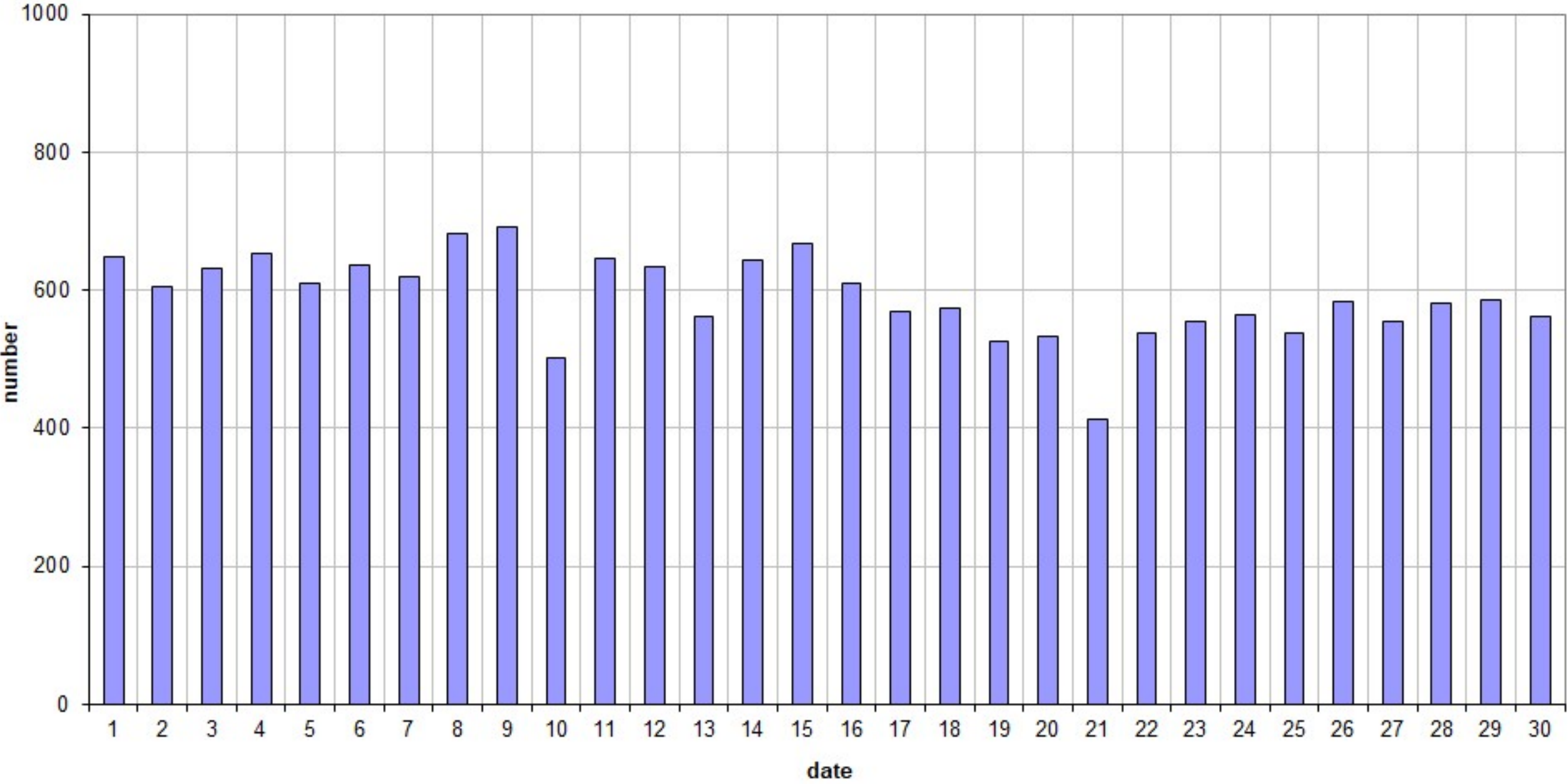
49.99MHz - RadioMeteors November 2025 daily totals of "all" reflections (automatic count_Mettel5_7Hz) Felix Verbelen (Kamphenhout)
