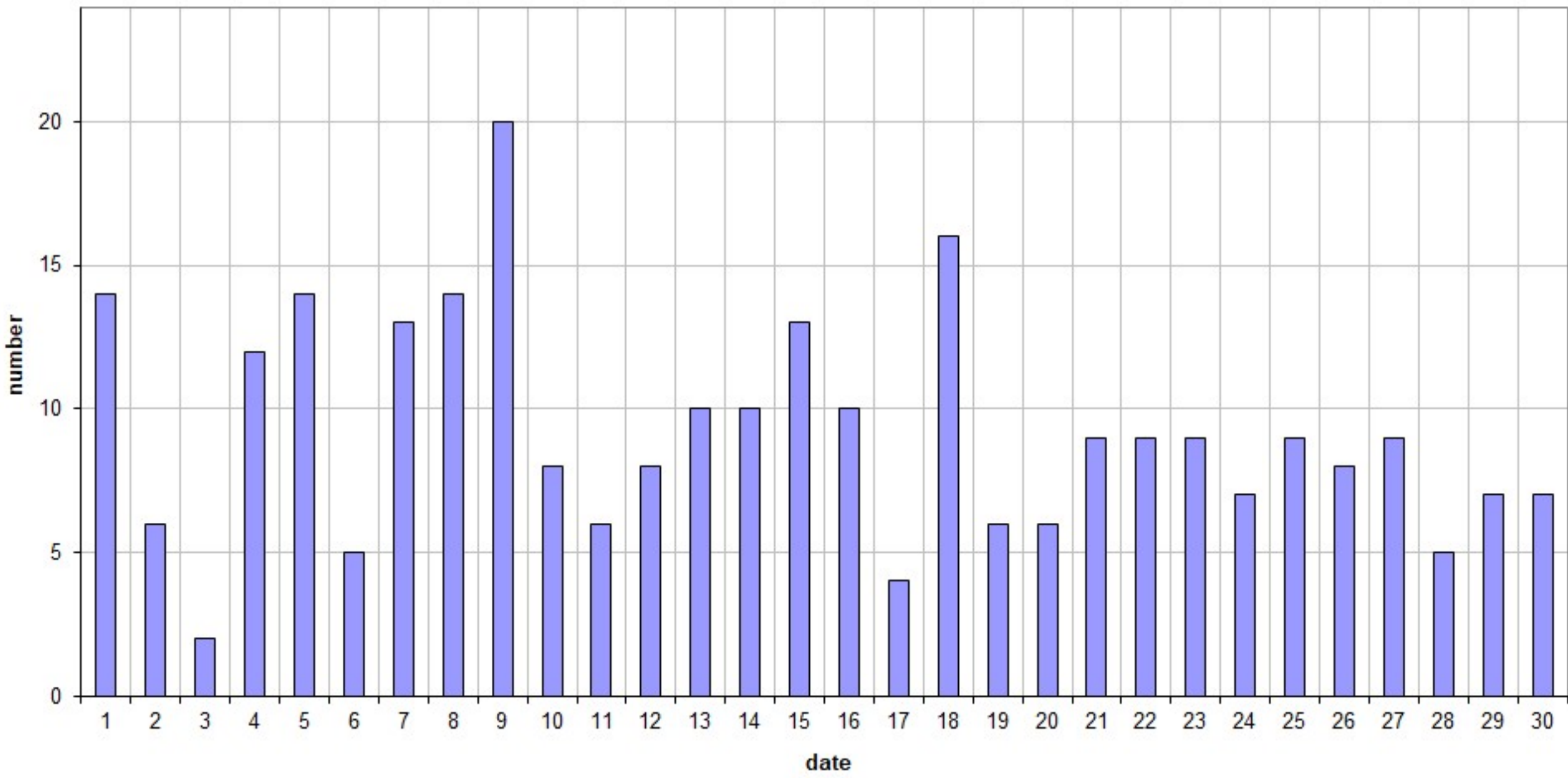
49.99MHz - RadioMeteors November 2025 daily totals of reflections longer than 10 seconds Felix Verbelen (Kamphenhout)
