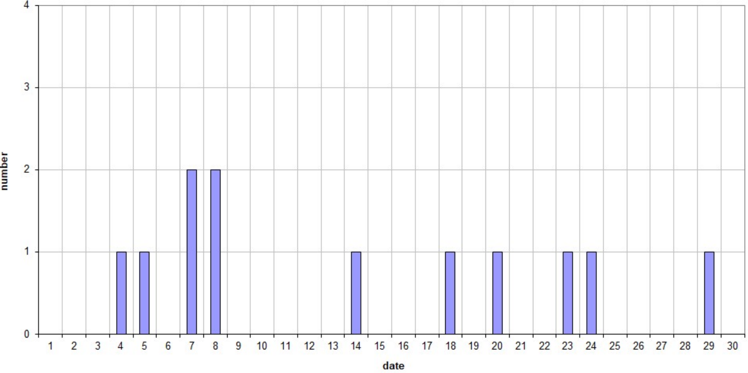
49.99MHz - RadioMeteors November 2025 daily totals of reflections longer than 1 minute Felix Verbelen (Kamphenhout)
