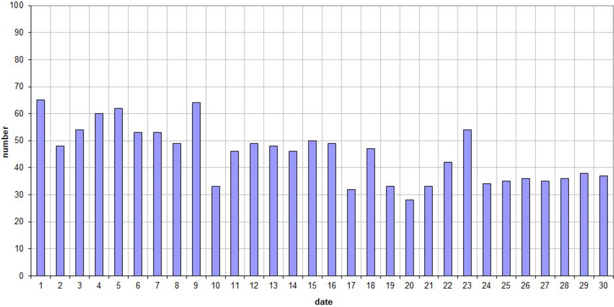
49.99MHz - RadioMeteors November 2025 daily totals of all overdense reflections Felix Verbelen (Kamphenhout)
