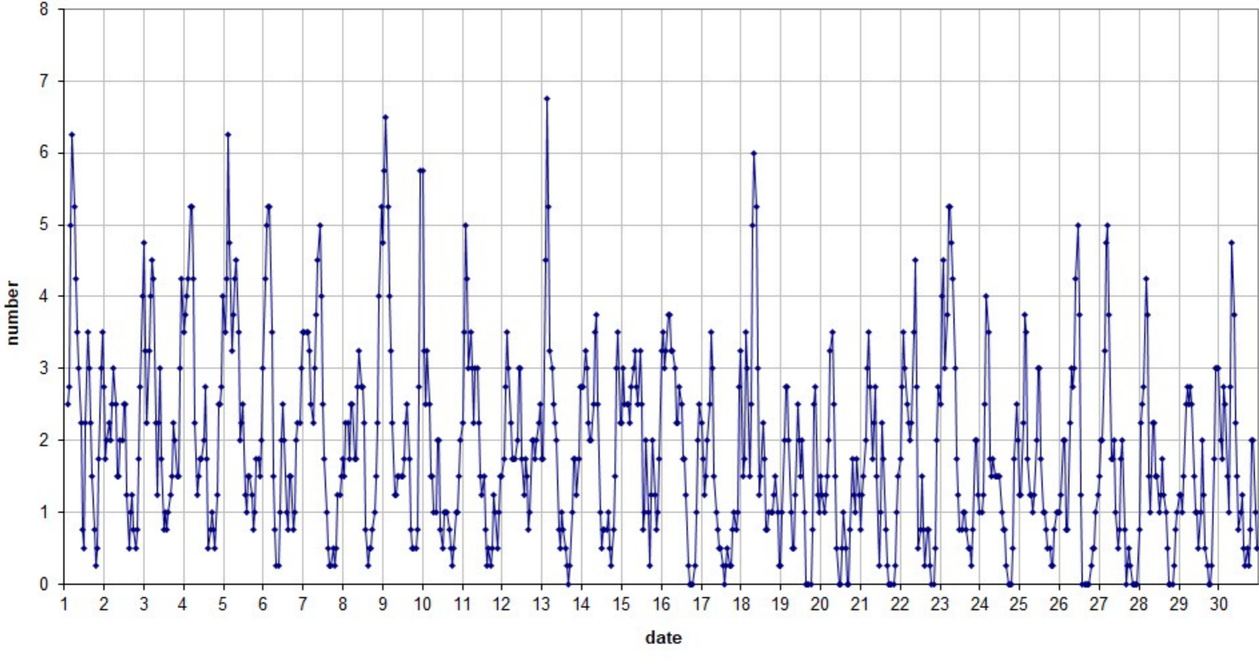
49.99MHz - RadioMeteors November 2025 number of overdense reflections per hour (weighted average) Felix Verbelen (Kampenhout)
