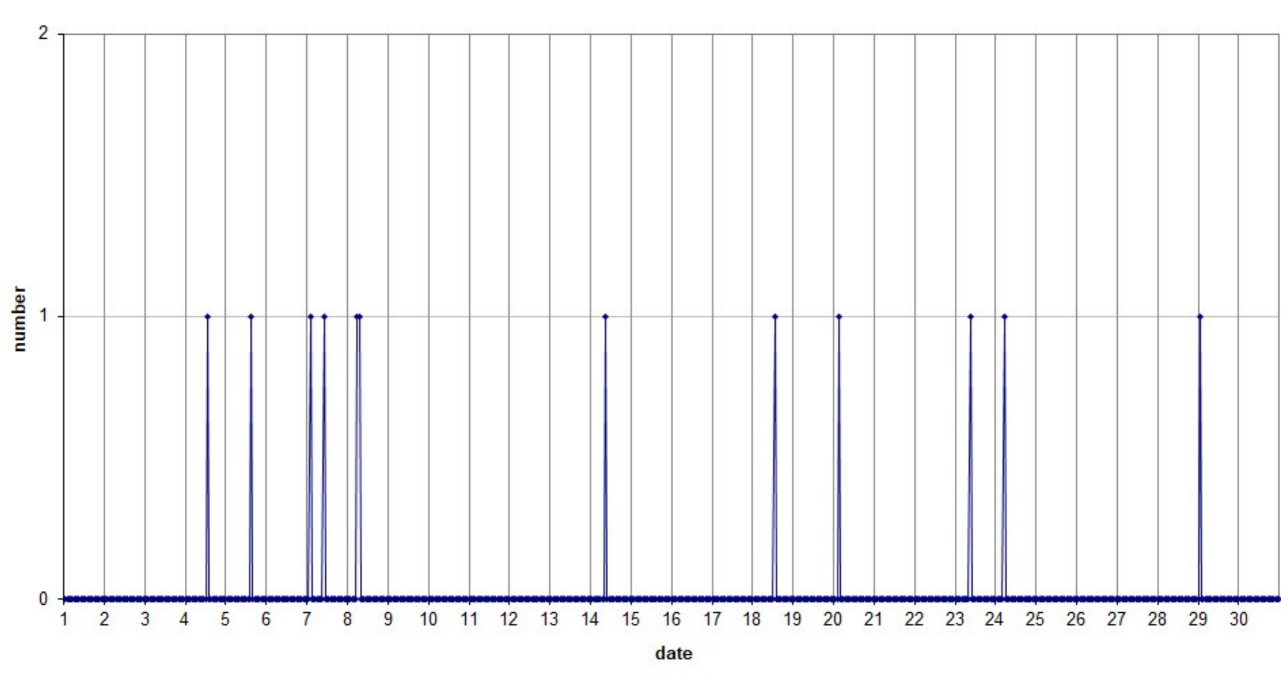
49.99MHz - RadioMeteors November 2025 hourly totals of overdense reflections longer than 1 minute Felix Verbelen (Kampenhout/BE)
