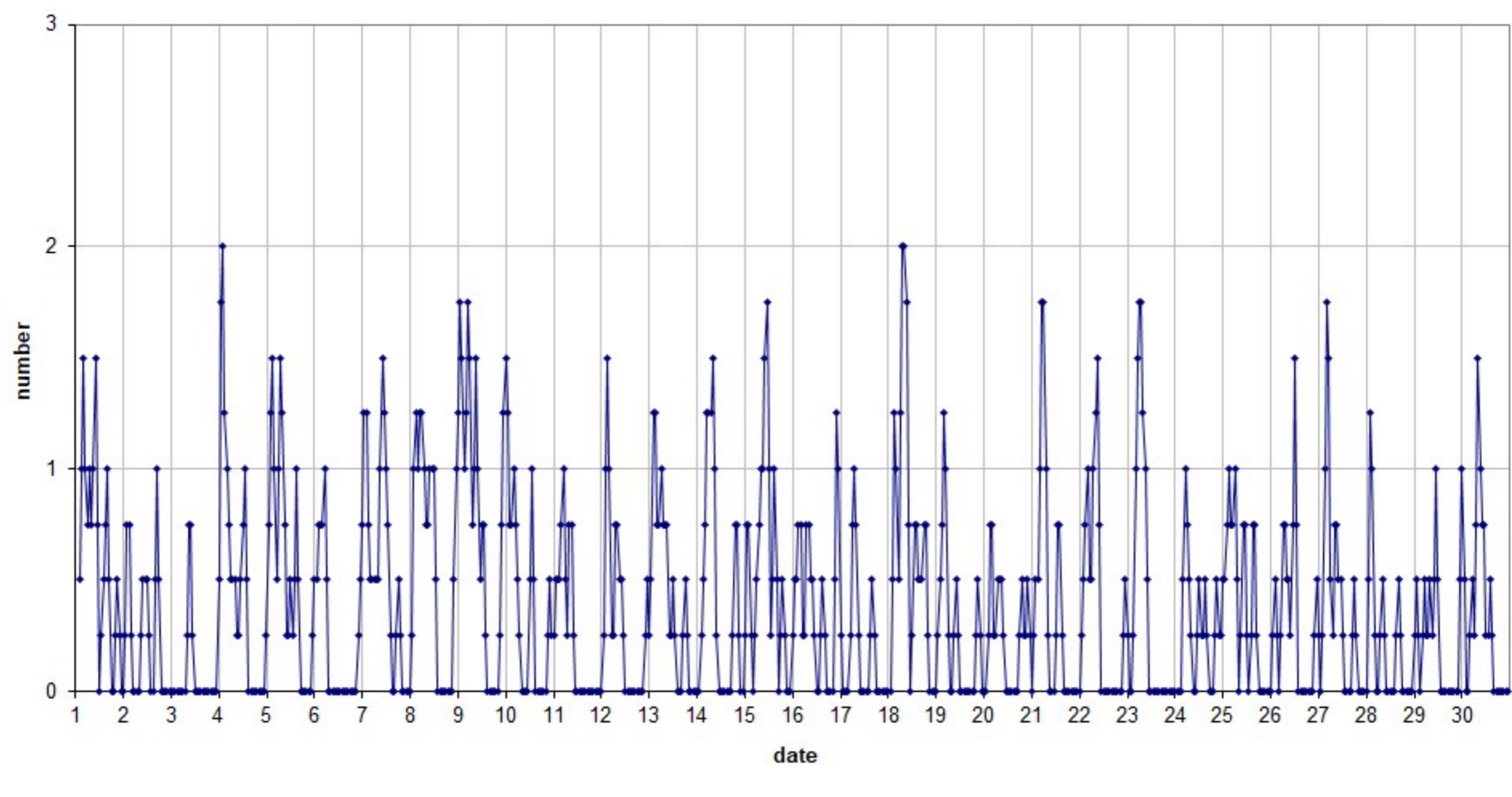
49.99MHz - RadioMeteors November 2025 number of reflections >10 seconds per hour (weighted average) Felix Verbelen (Kampenhout)
