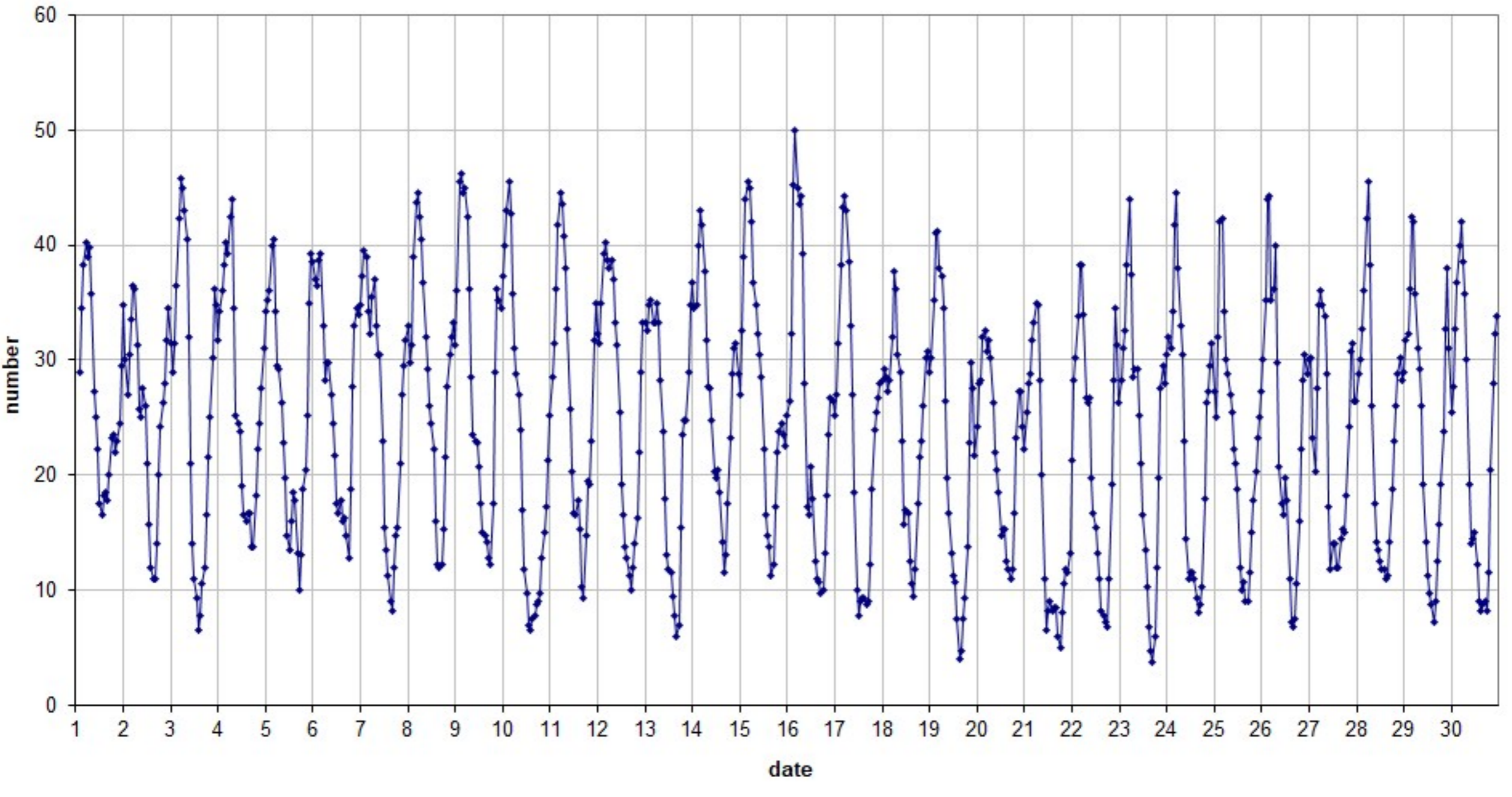
49.99 MHz - RadioMeteors November 2025 number of "all" reflections per hour (weighted average) (automatic count_Metel5_7Hz) Felix Verbelen (Kampenhout)
