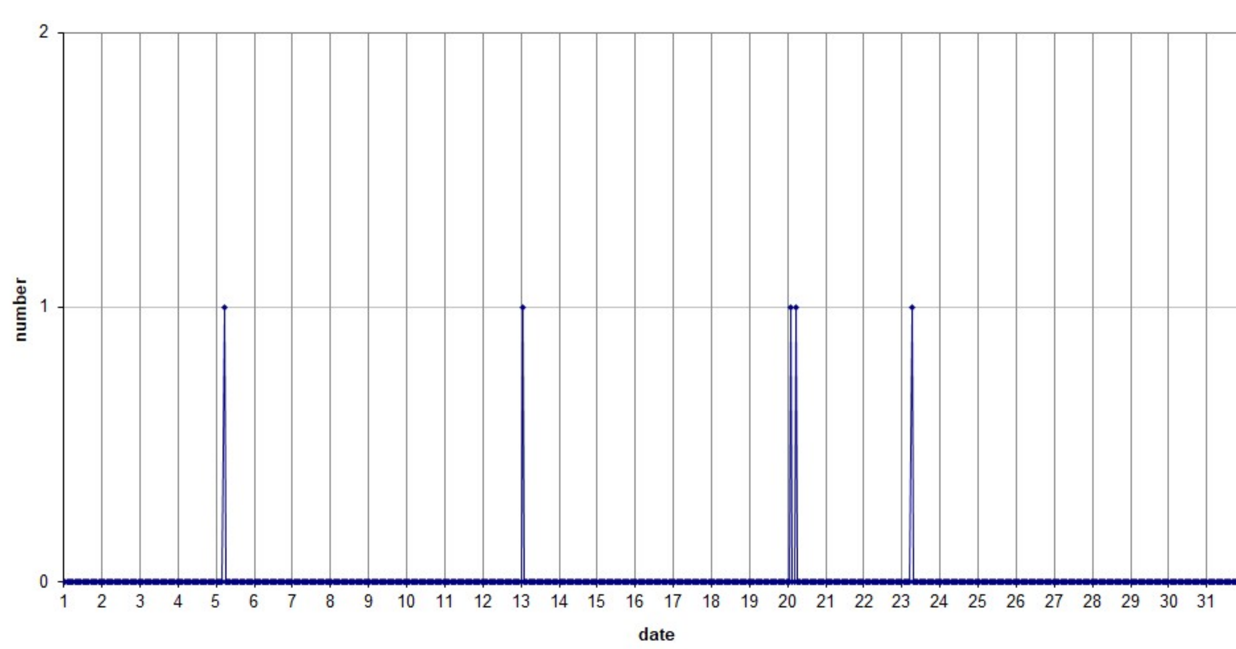
49.99MHz - RadioMeteors January 2026 hourly totals of overdense reflections longer than 1 minute Felix Verbelen (Kampenhout/BE)
