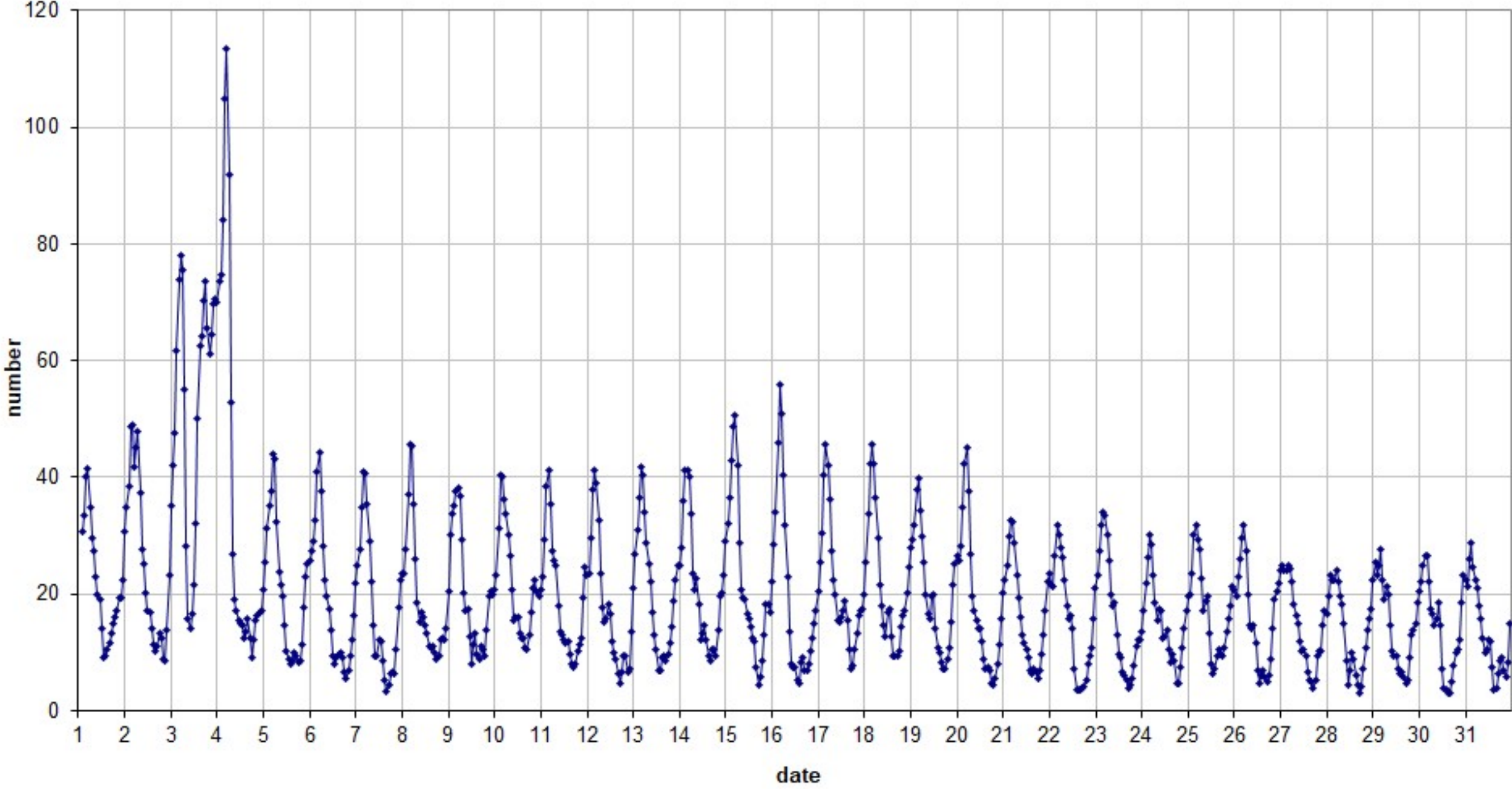
49.99 MHz - RadioMeteors January 2026 number of "all" refections per hour (weighted average) (automatic count_Mettel5_7Hz) Felix Verbelen (Kampenhout)
