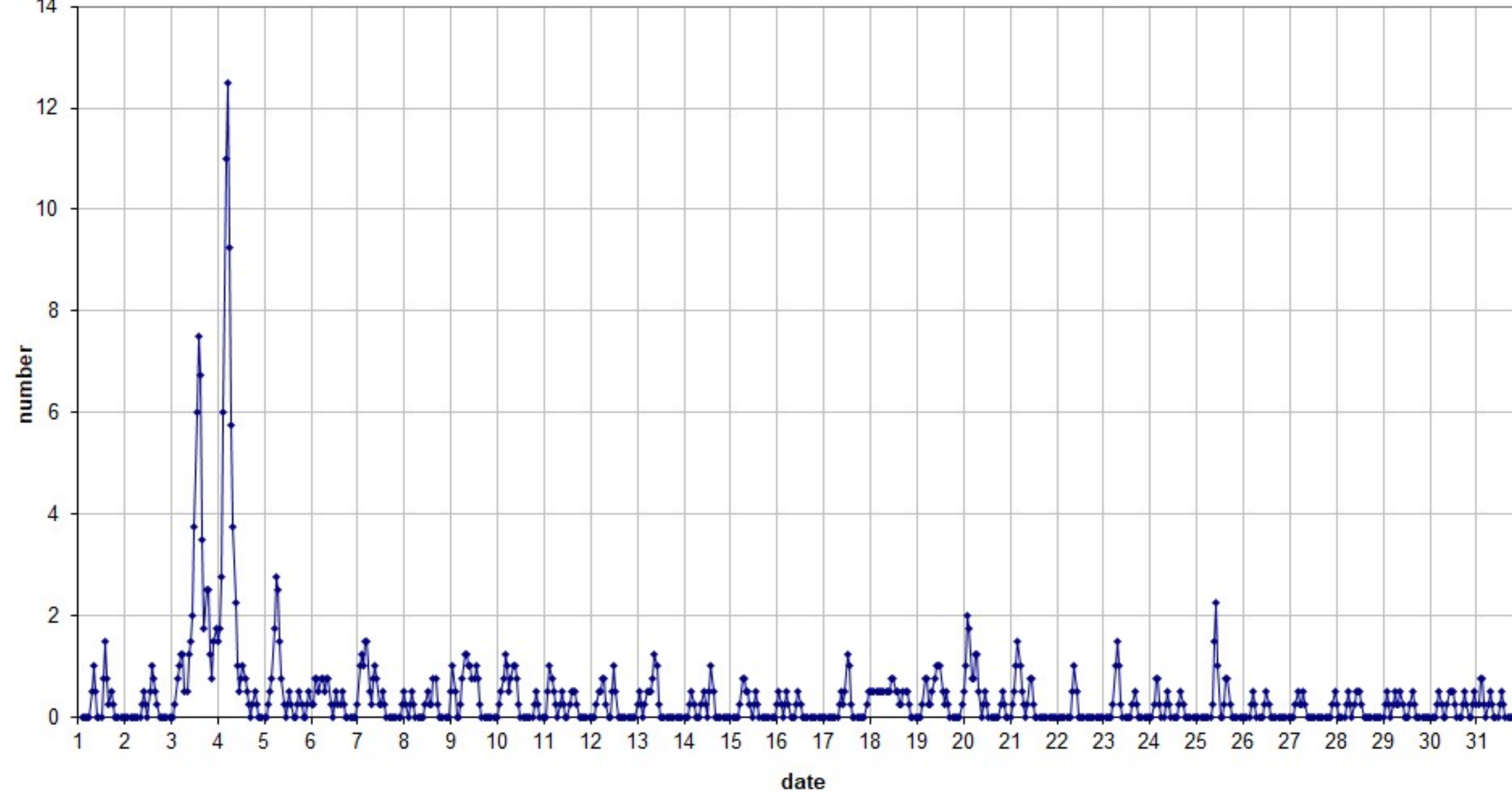
49.99MHz - RadioMeteors January 2026 number of reflections >10 seconds per hour (weighted average) Felix Verbelen (Kampenhout)
