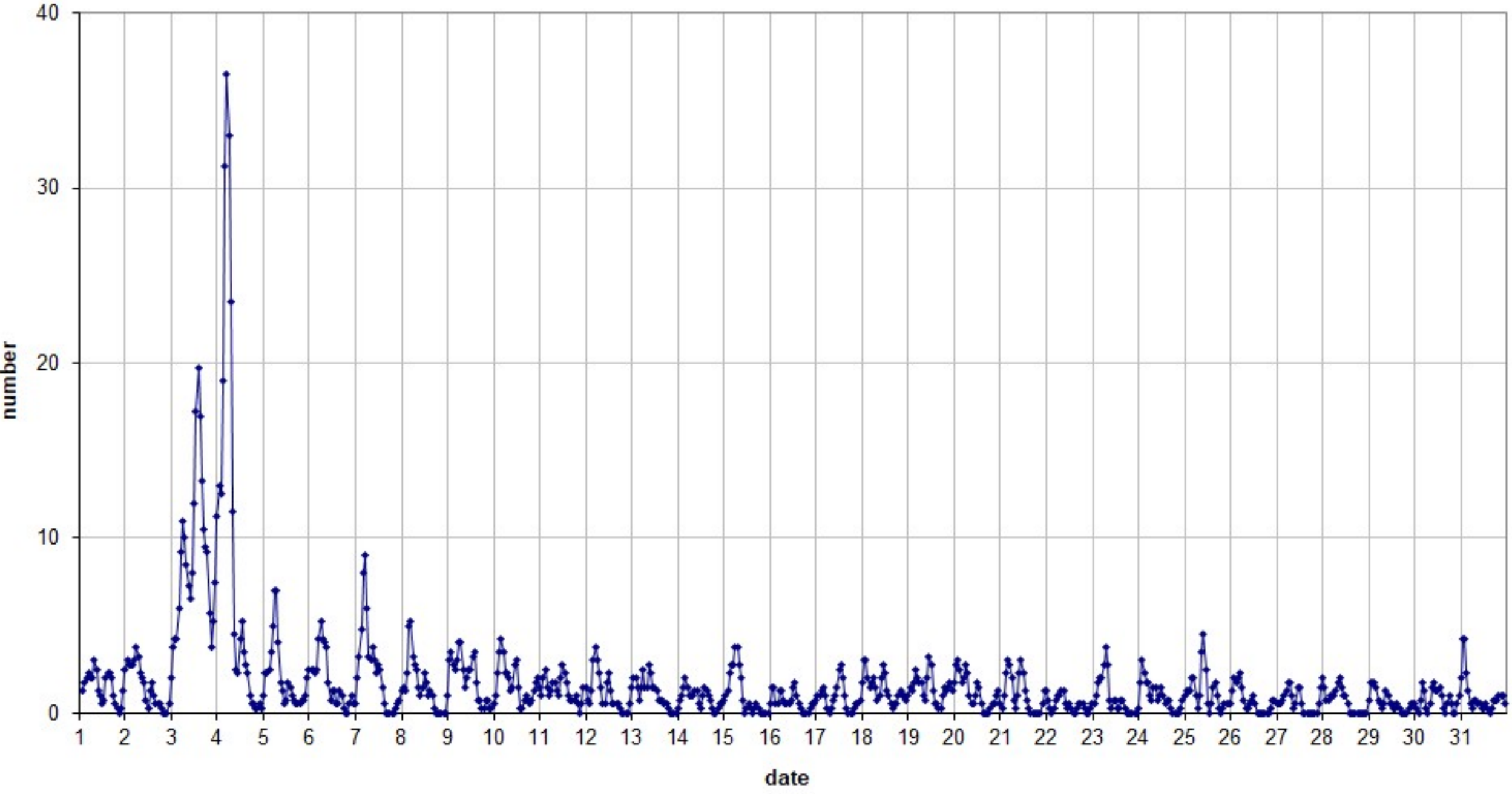
49.99MHz - RadioMeteors January 2026 number of overdense reflections per hour (weighted average) Felix Verbelen (Kampenhout)
