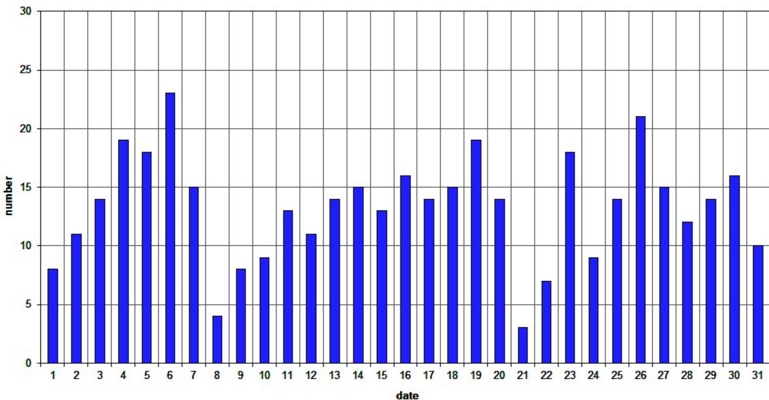
49.99MHz - RadioMeteors March 2026 daily totals of all overdense reflections Felix Verbelen (Kampenhout)
