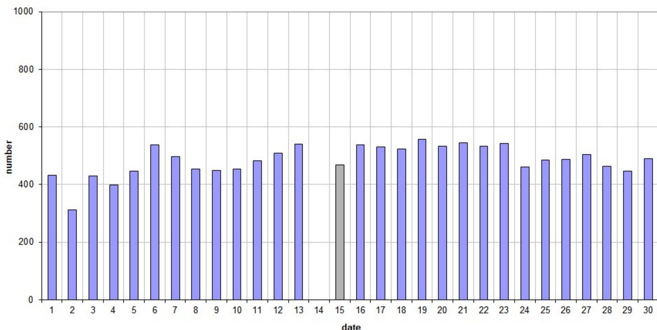
49.99MHz - RadioMeteors April 2026 daily totals of "all" reflections (automatic count_Mettel5_7Hz) Felix Verbelen (Kampenhout)
