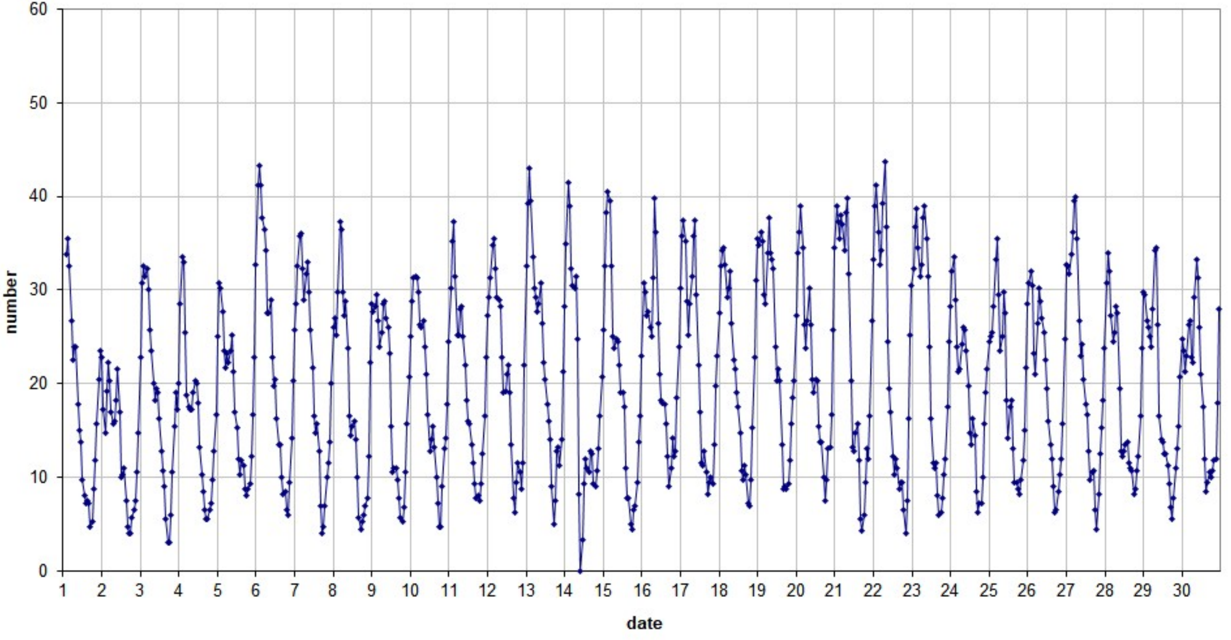
49.99 MHz - RadioMeteors April 2026 number of "all" reflections per hour (weighted average) (automatic count_MetteI5_7Hz) Felix Verbelen (Kamphenhout)
