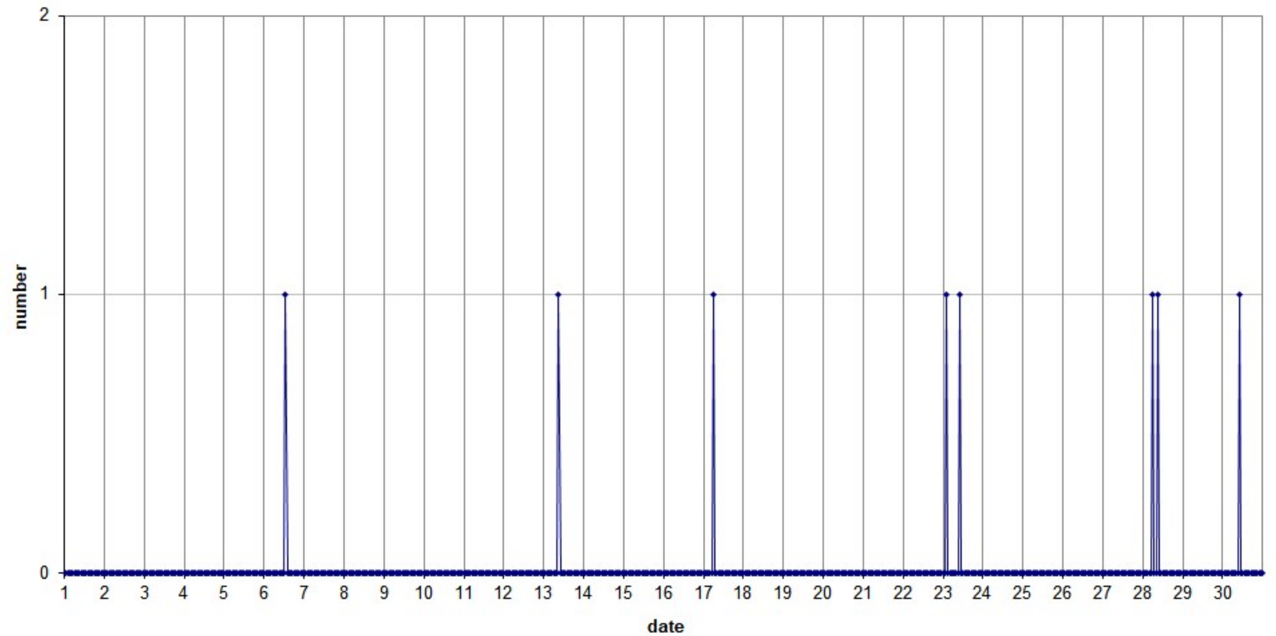
49.99MHz - RadioMeteors April 2026 hourly totals of overdense reflections longer than 1 minute Felix Verbelen (Kamphenhout/BE)
