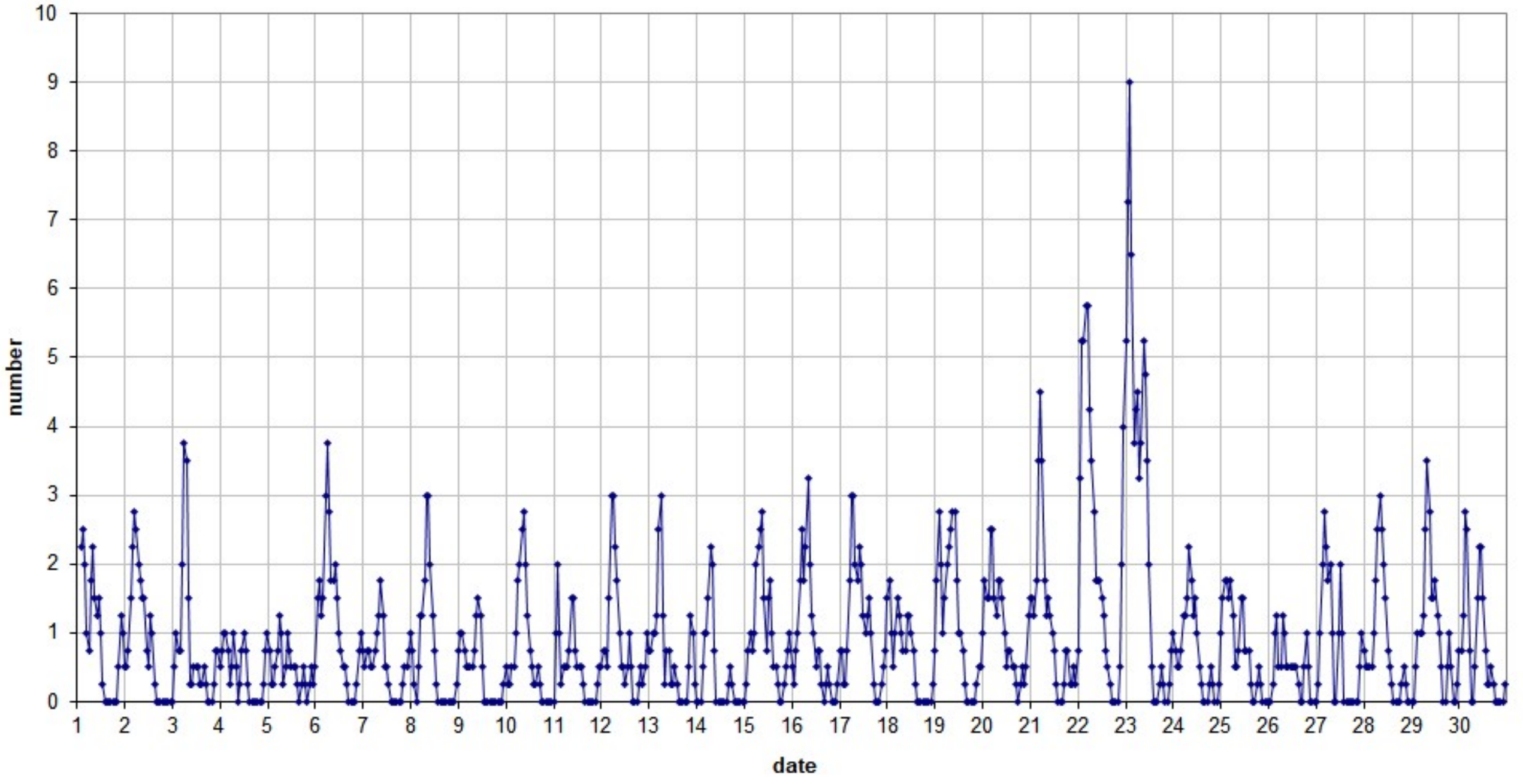
49.99MHz - RadioMeteors April 2026 number of overdense reflections per hour (weighted average) Felix Verbelen (Kamphenhout)
