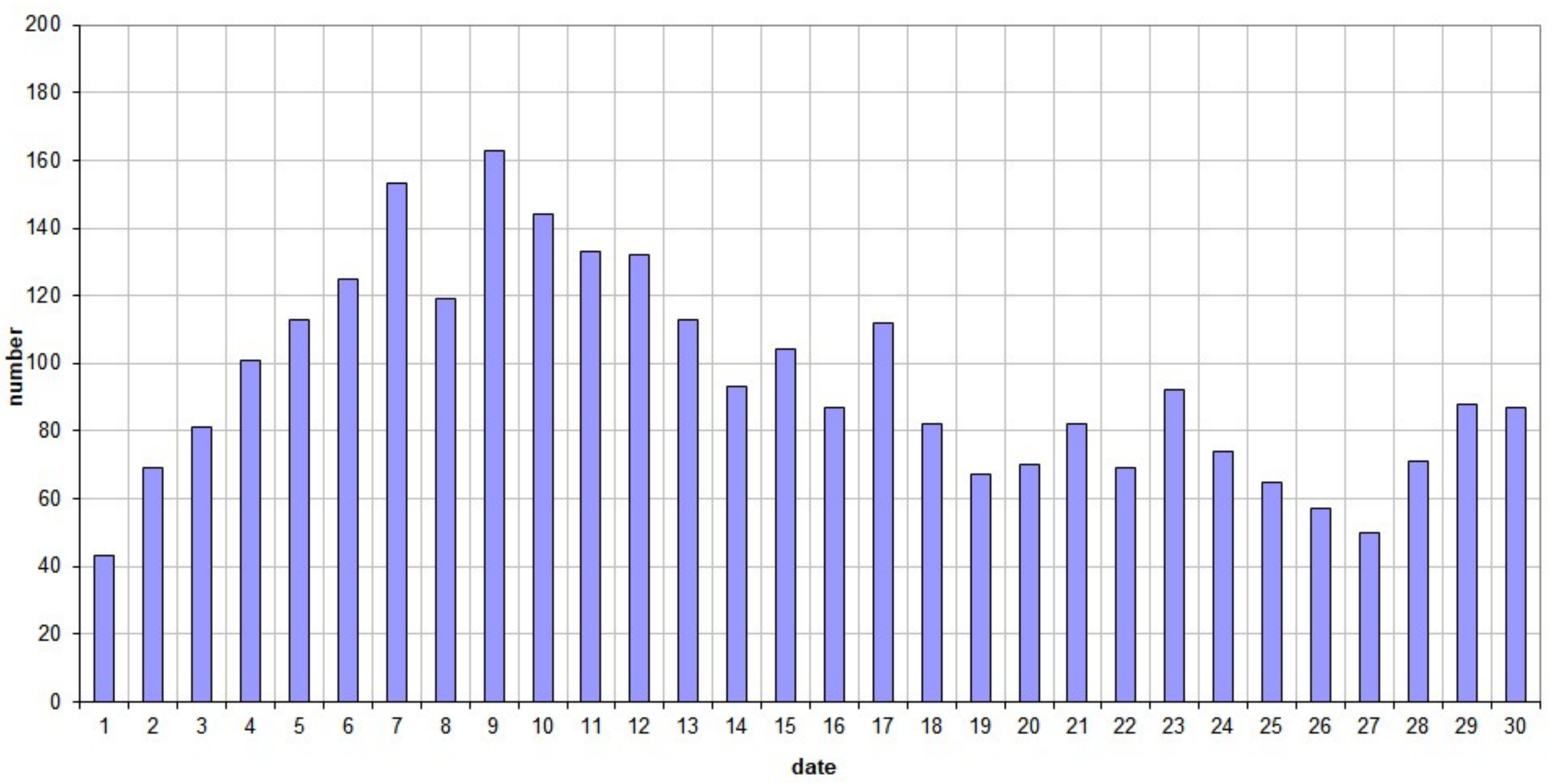
49.99MHz - RadioMeteors June 2026 daily totals of all overdense reflections Felix Verbelen (Kampenhout)
