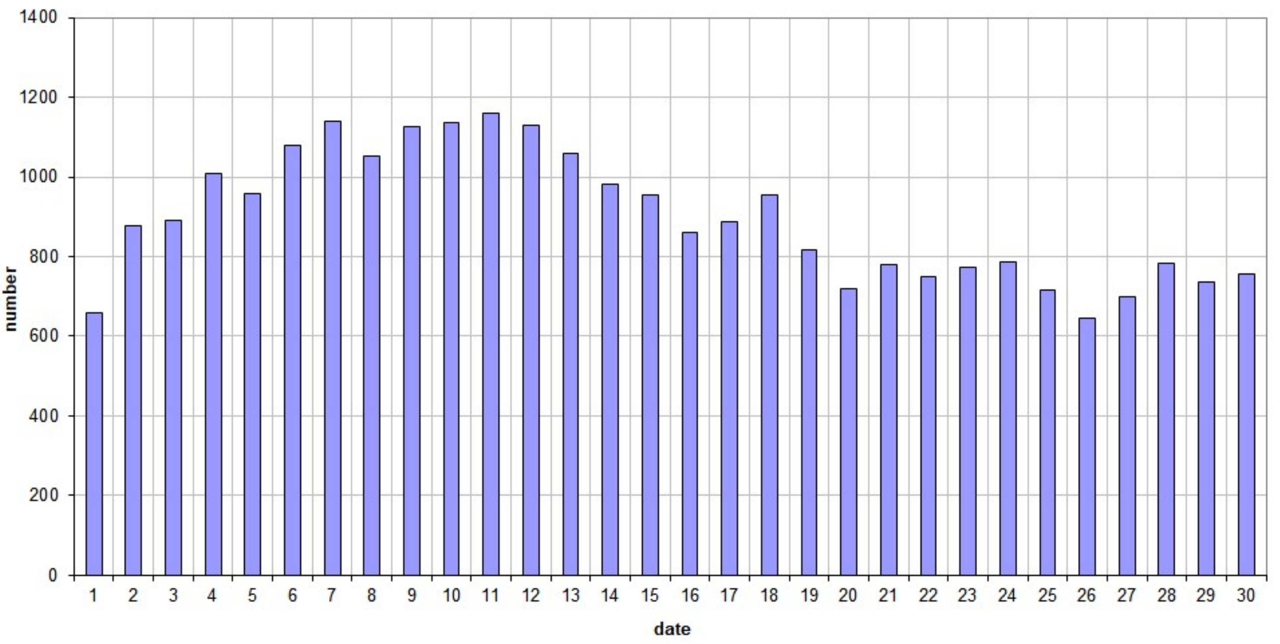
49.99MHz - RadioMeteors June 2026 daily totals of "all" reflections (automatic count_Mette15_7Hz) Felix Verbelen (Kampenhout)
