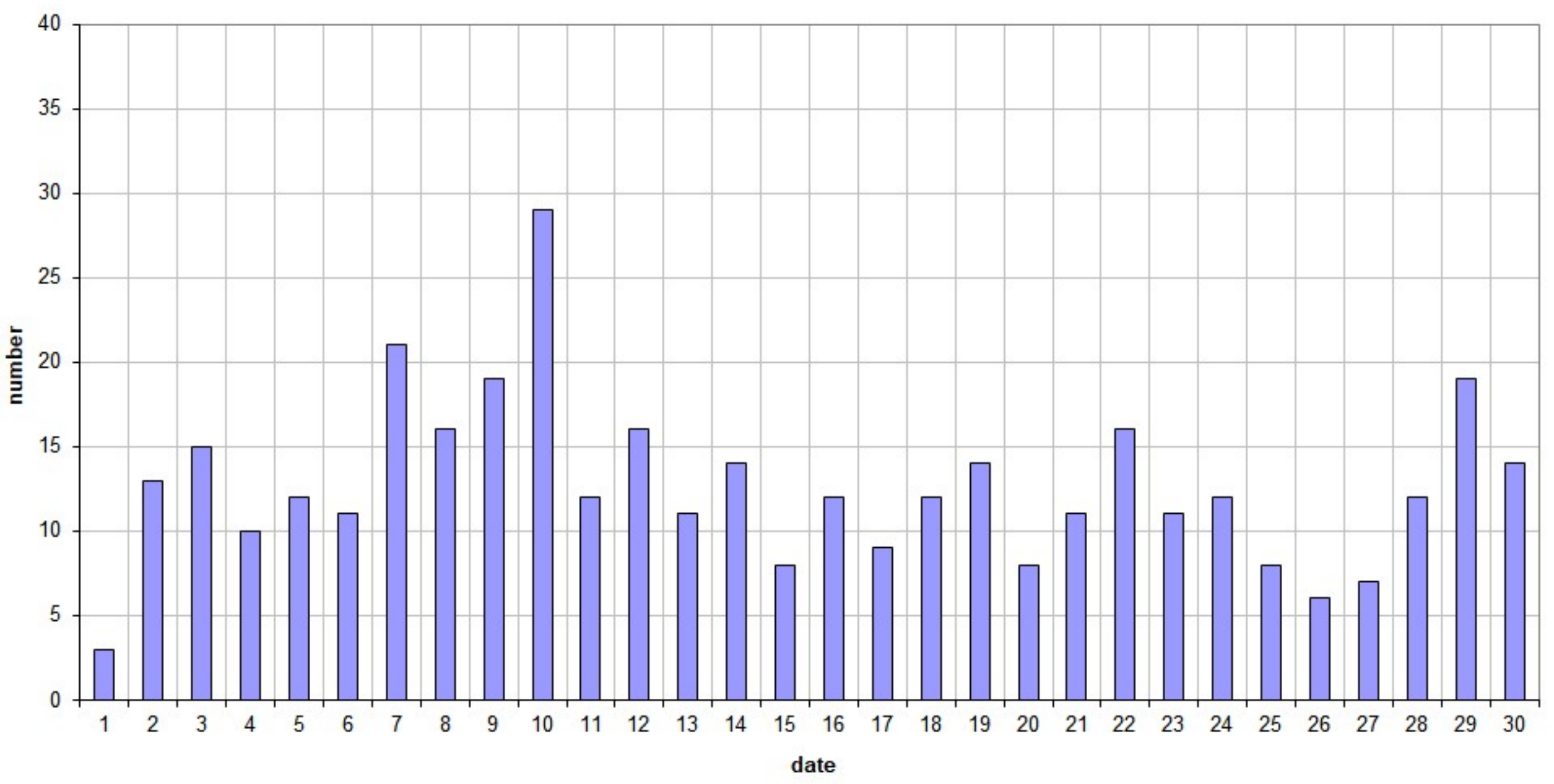
49.99MHz - RadioMeteors June 2026 daily totals of reflections longer than 10 seconds Felix Verbelen (Kampenhout)
