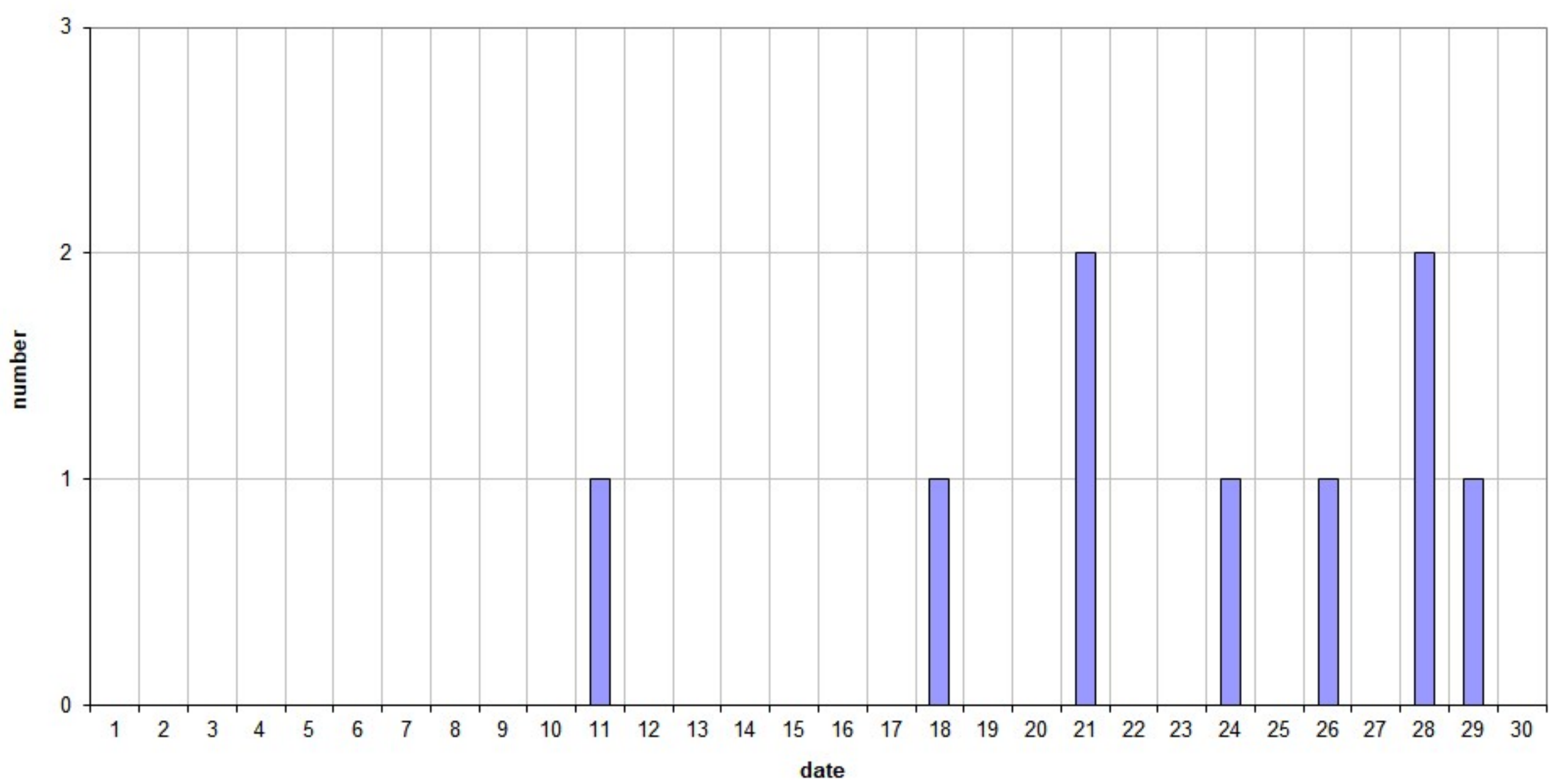
49.99MHz - RadioMeteors June 2026 daily totals of reflections longer than 1 minute Felix Verbelen (Kampenhout)
