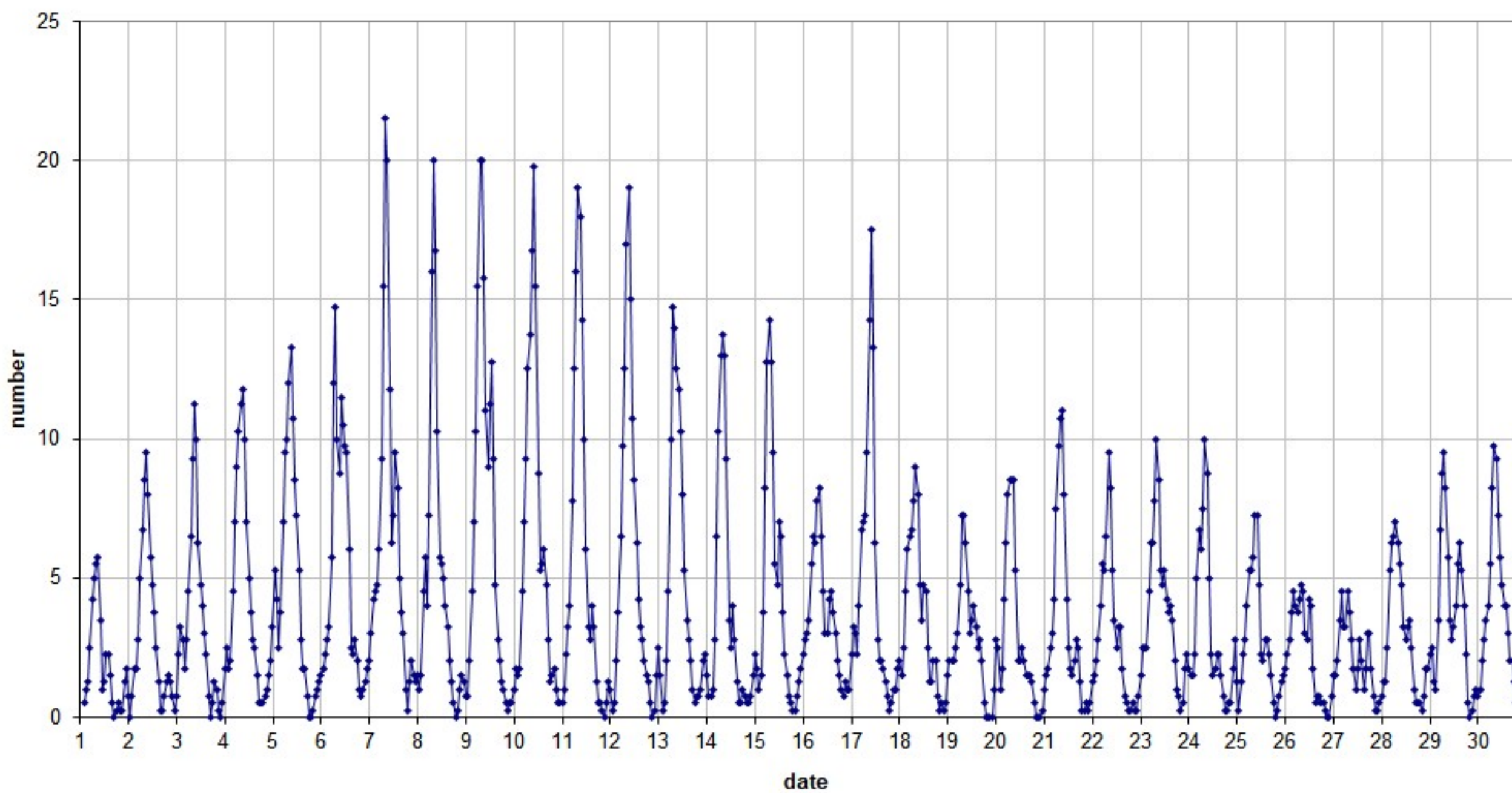
49.99MHz - RadioMeteors June 2026 number of overdense reflections per hour (weighted average) Felix Verbelen (Kamphenhout)
