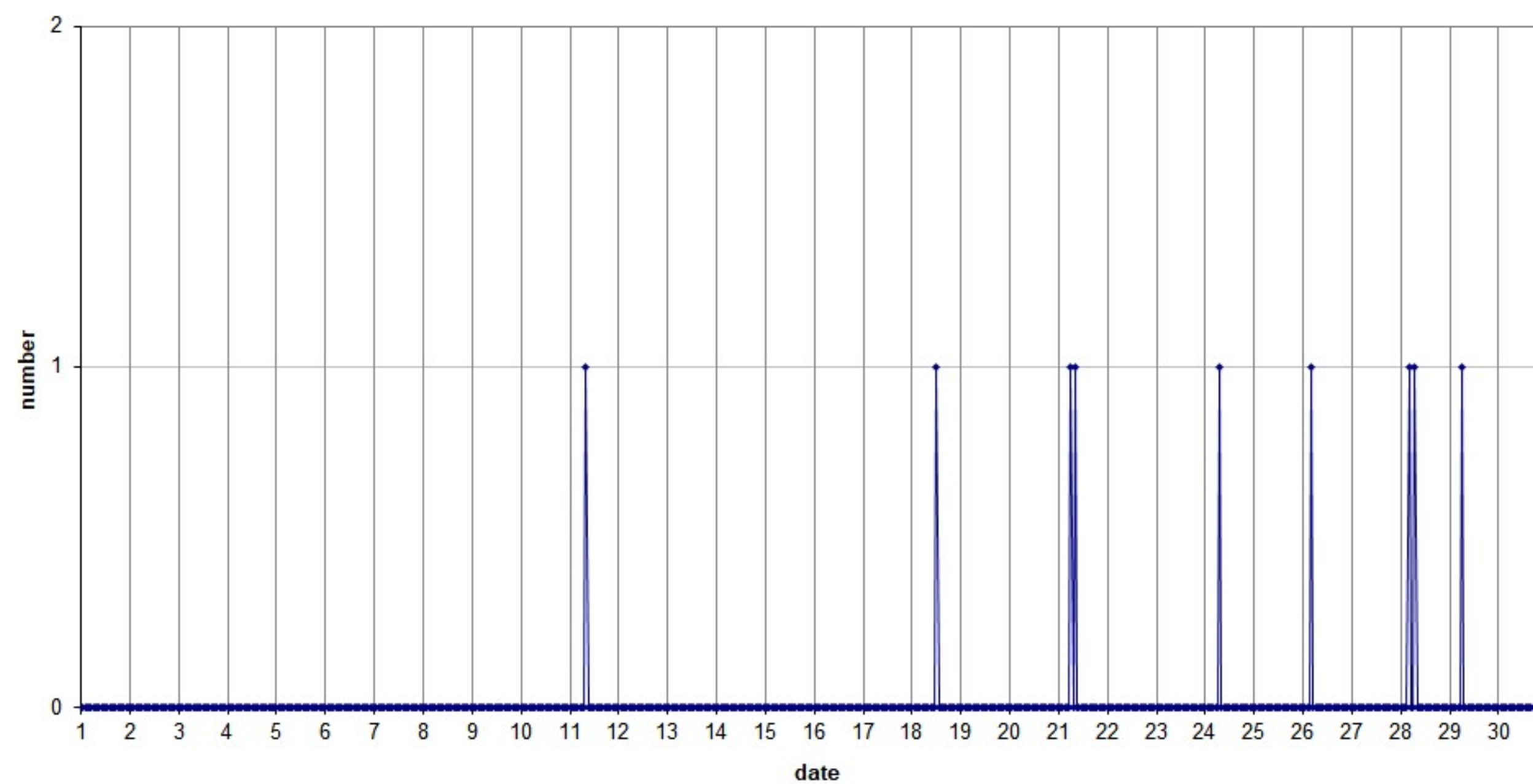
49.99MHz - RadioMeteors June 2026 hourly totals of overdense reflections longer than 1 minute Felix Verbelen (Kamphenhout/BE)
