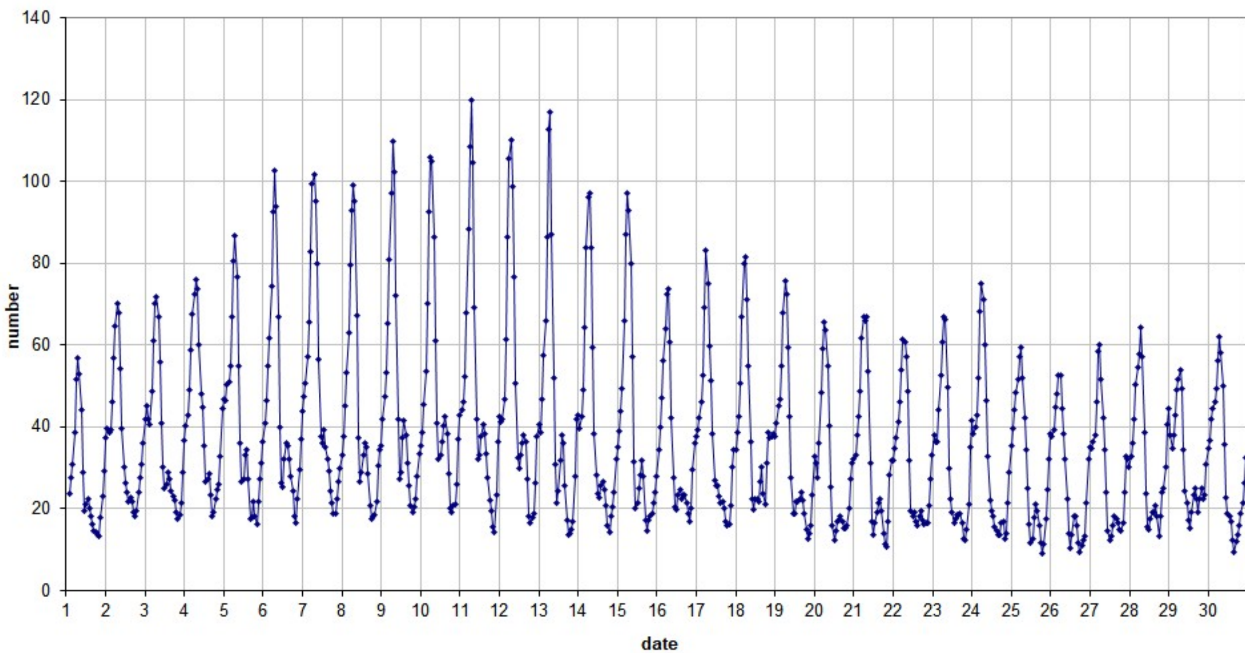
49.99 MHz - RadioMeteors June 2026 number of "all" reflections per hour (weighted average) (automatic count_Mettel5_7Hz) Felix Verbelen (Kamphenhout)
