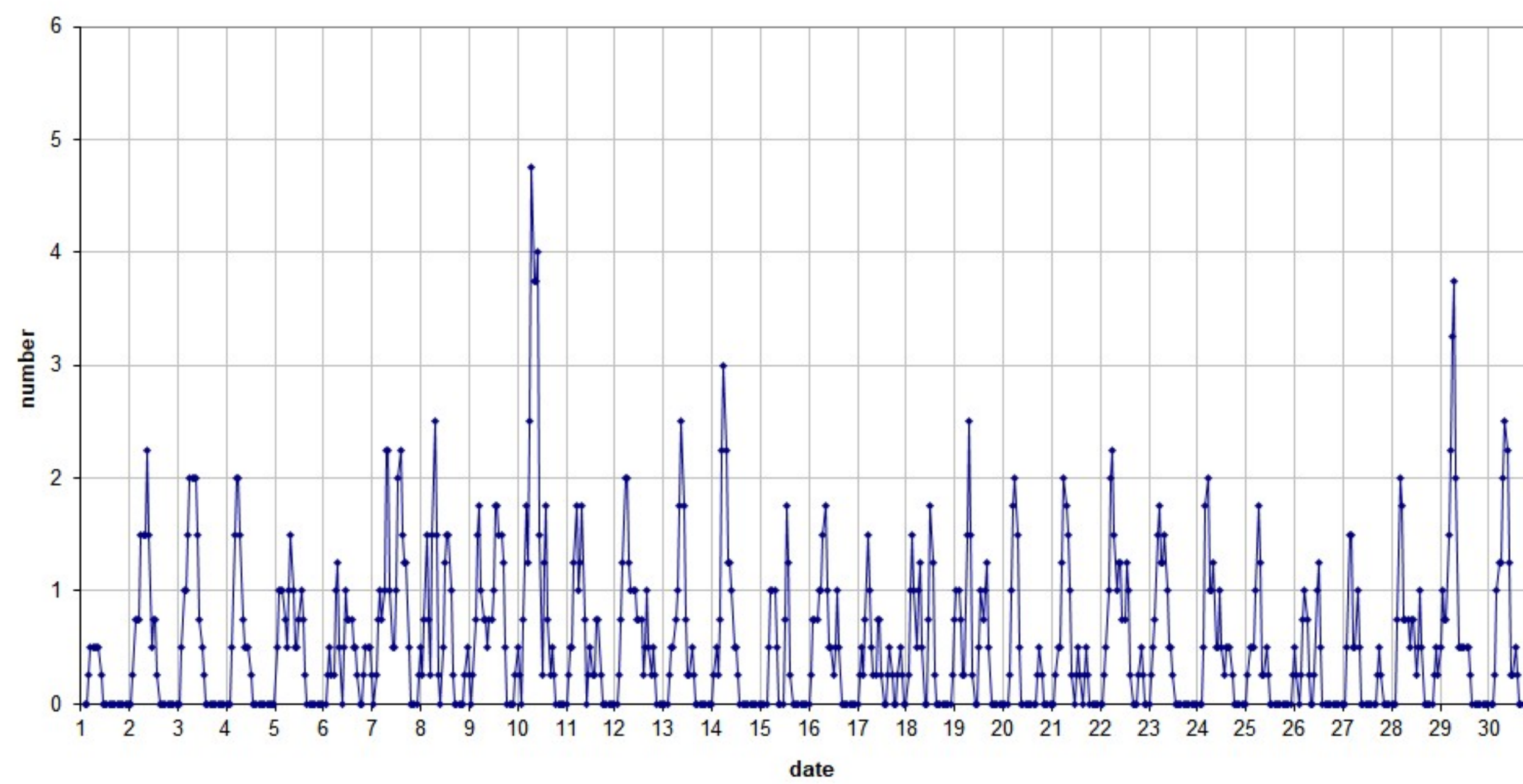
49.99MHz - RadioMeteors June 2026 number of reflections >10 seconds per hour (weighted average) Felix Verbelen (Kamphenhout)
