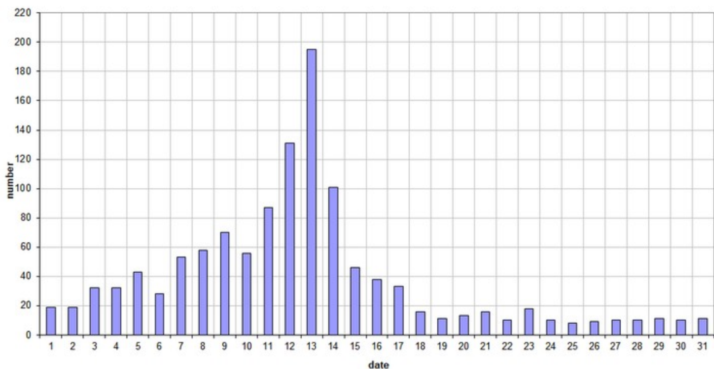
49.99MHz - RadioMeteors August 2026 daily totals of reflections longer than 10 seconds Felix Verbelen (Kamphenhout)
