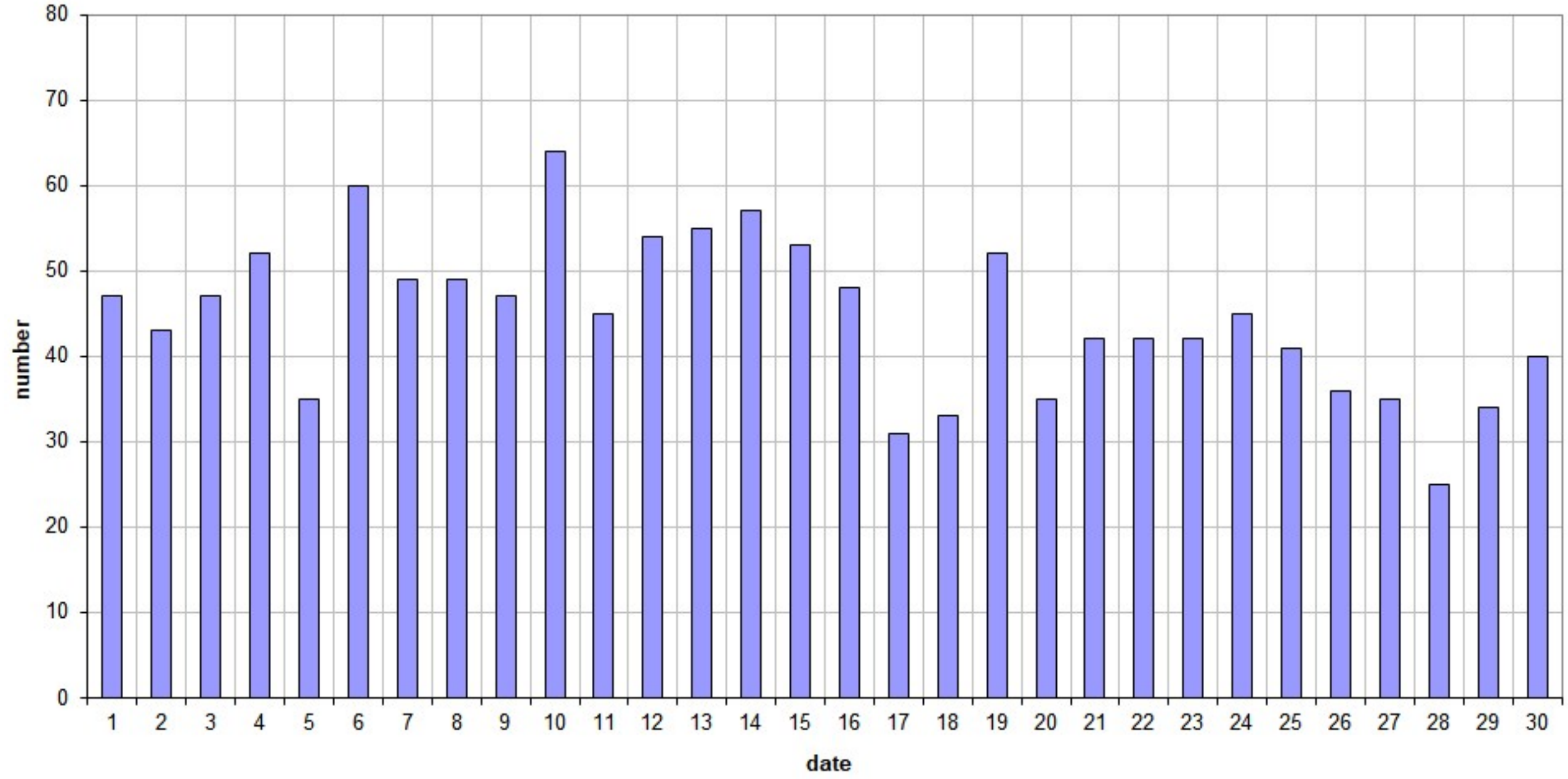
49.99MHz - RadioMeteors September 2026 daily totals of all overdense reflections Felix Verbelen (Kampenhout)
