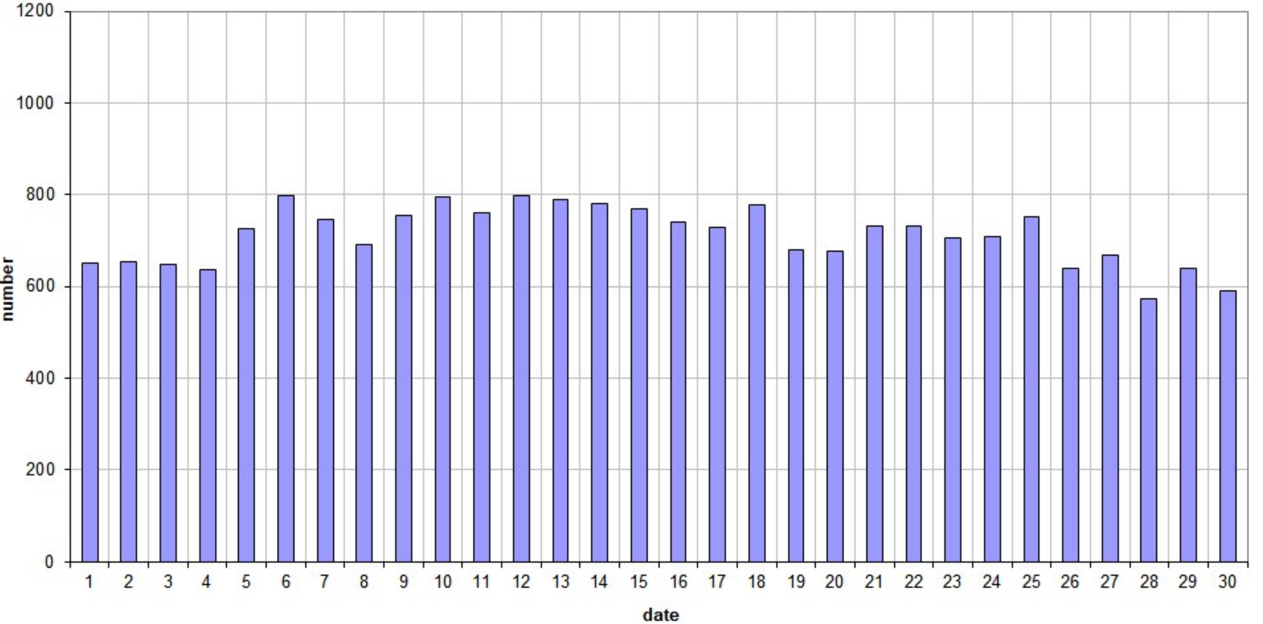
49.99MHz - RadioMeteors September 2026 daily totals of "all" reflections (automatic count_Mettel5_7Hz) Felix Verbelen (Kampenhout)
