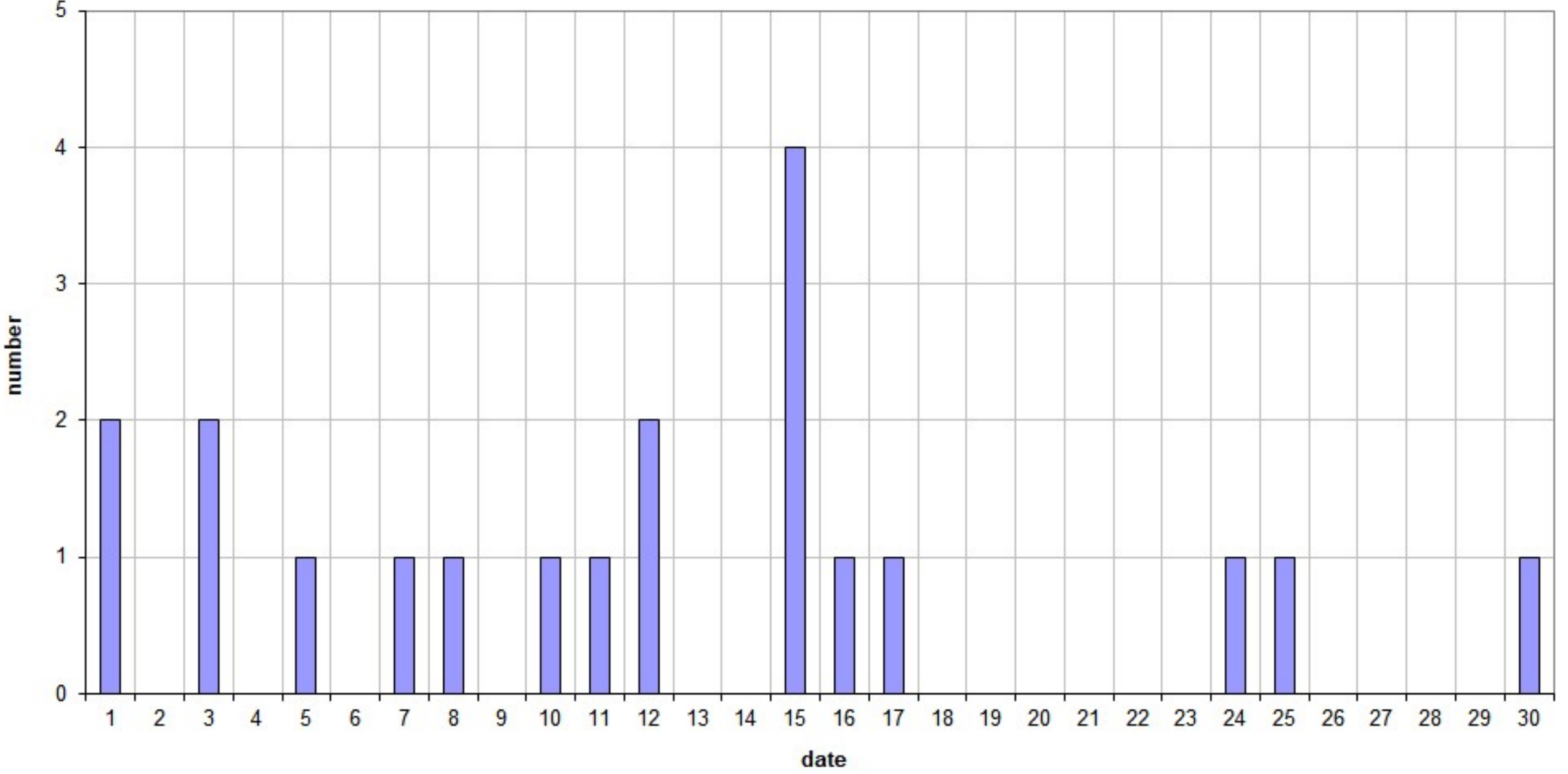
49.99MHz - RadioMeteors September 2026 daily totals of reflections longer than 1 minute Felix Verbelen (Kampenhout)
