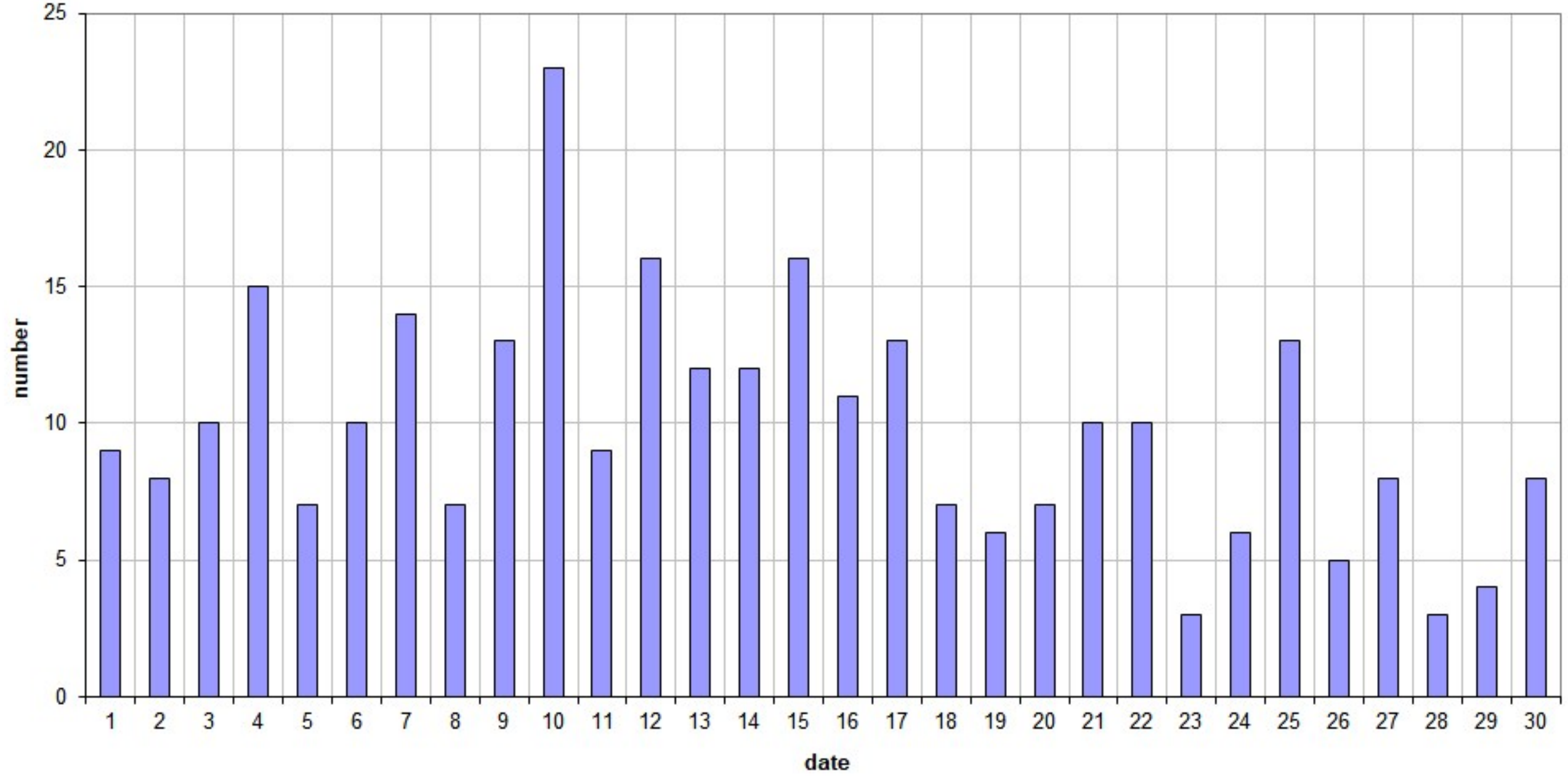
49.99MHz - RadioMeteors September 2026 daily totals of reflections longer than 10 seconds Felix Verbelen (Kampenhout)
