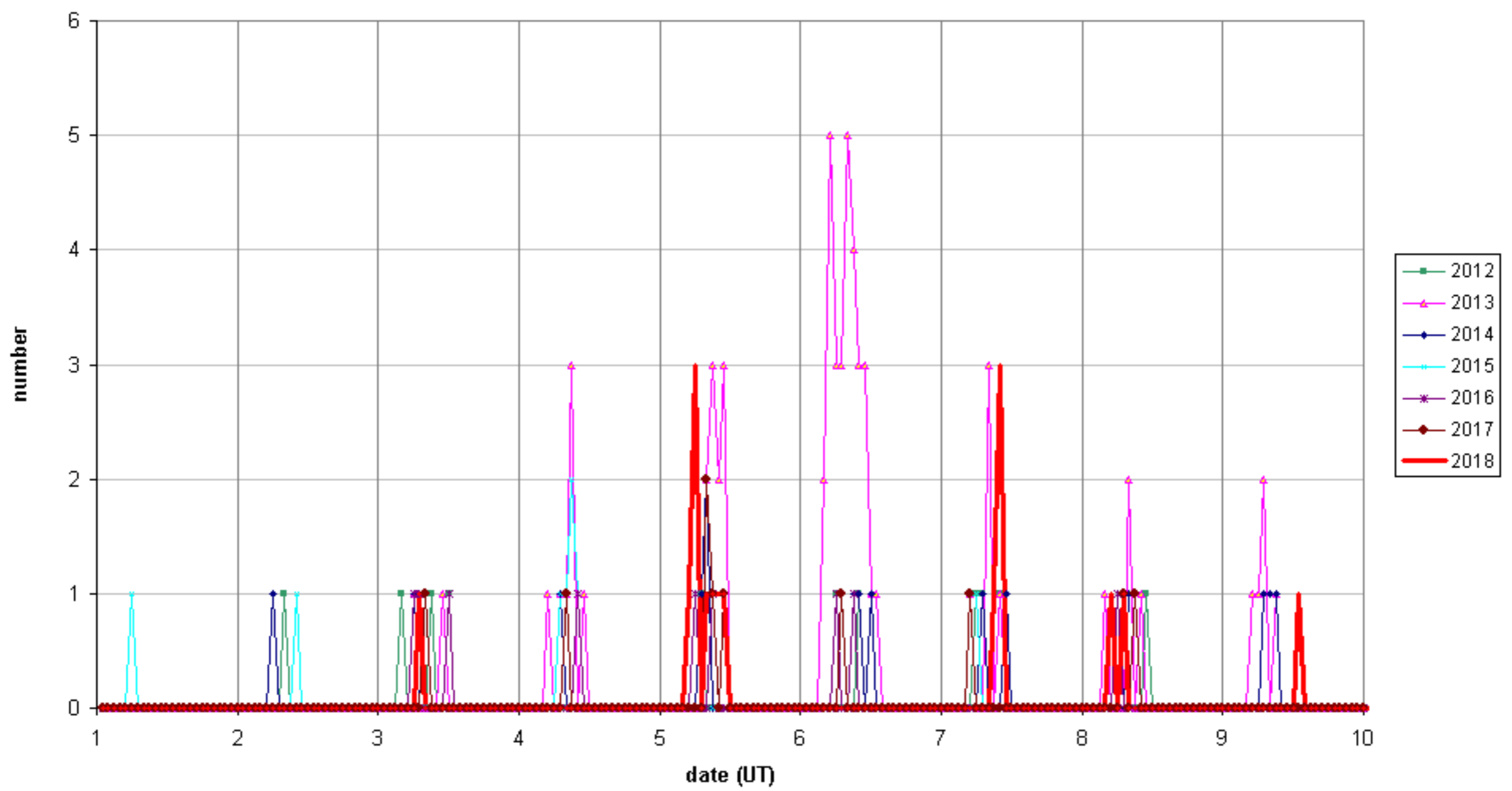
ETA_2012-2018_49.99 MHz_FV/BEKAMP(Kampenhout) manually counted overdense reflections longer than 1 minute
