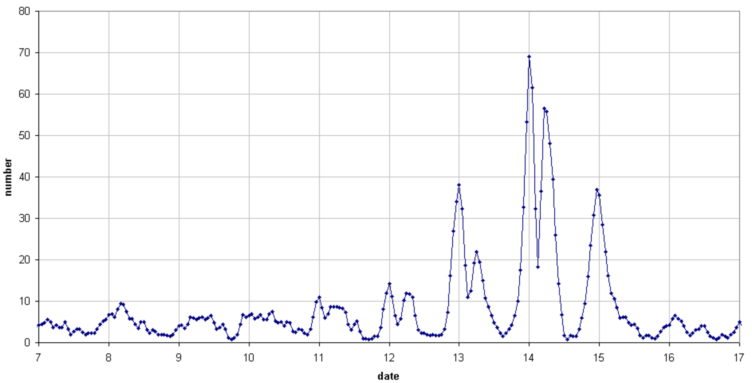
49.99MHz - GEMINIDS December 2018 number of overdense reflections per hour (weighted average) Felix Verbelen (Kampenhout)
