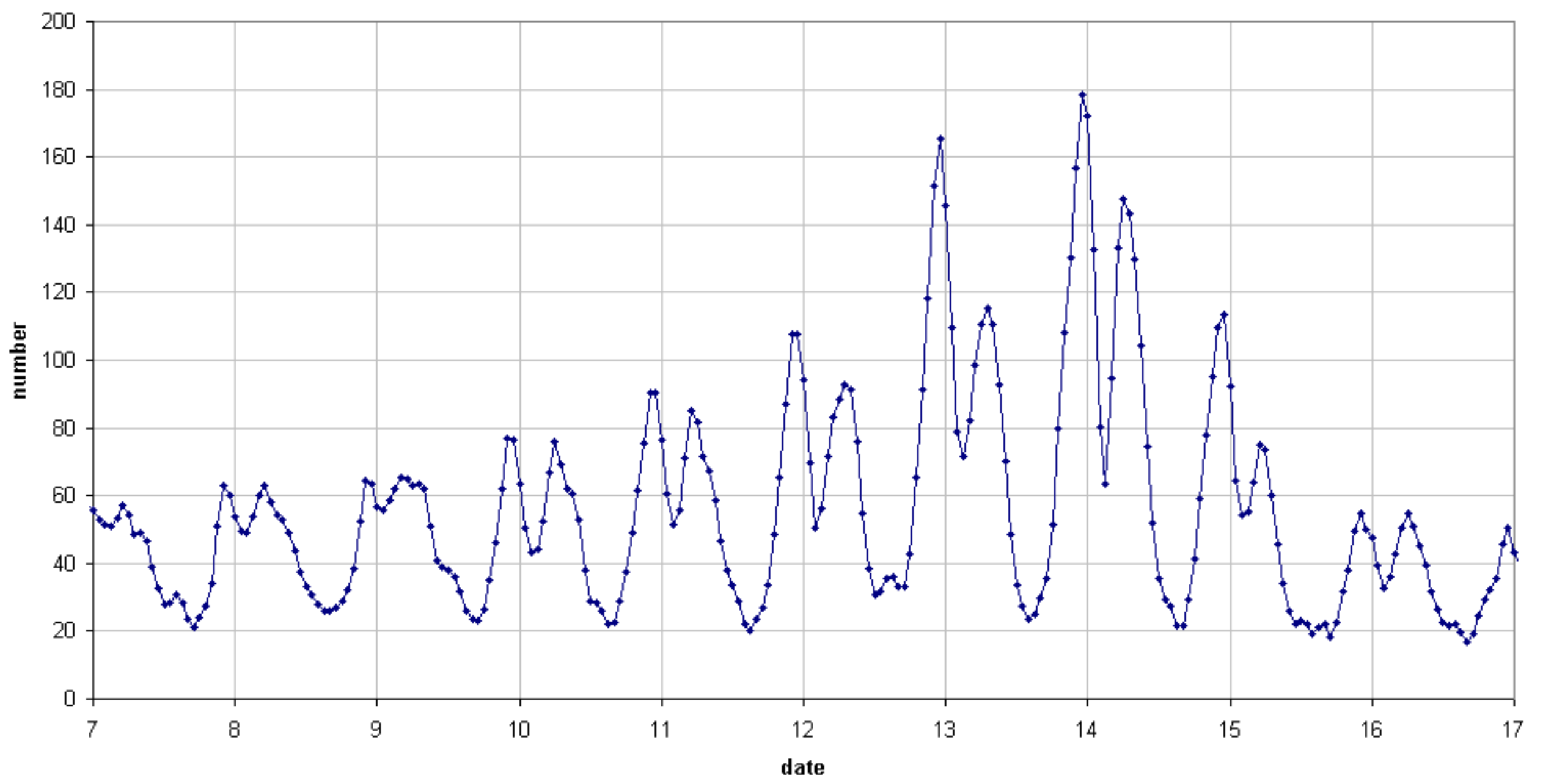
49.99 MHz - GEMINIDS December 2018 number of "all" reflections per hour (weighted average) (automatic count_Mette16_7Hz) Felix Verbelen (Kampenhout)
