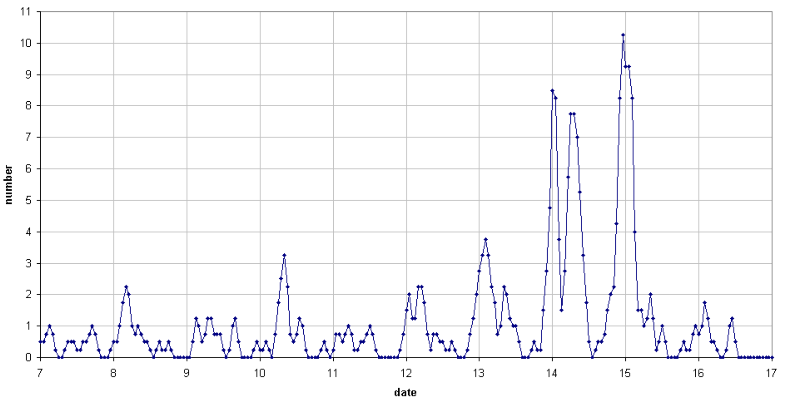
49.99MHz - GEMINIDS December 2018 number of reflections >10 seconds per hour (weighted average) Felix Verbelen (Kampenhout)
