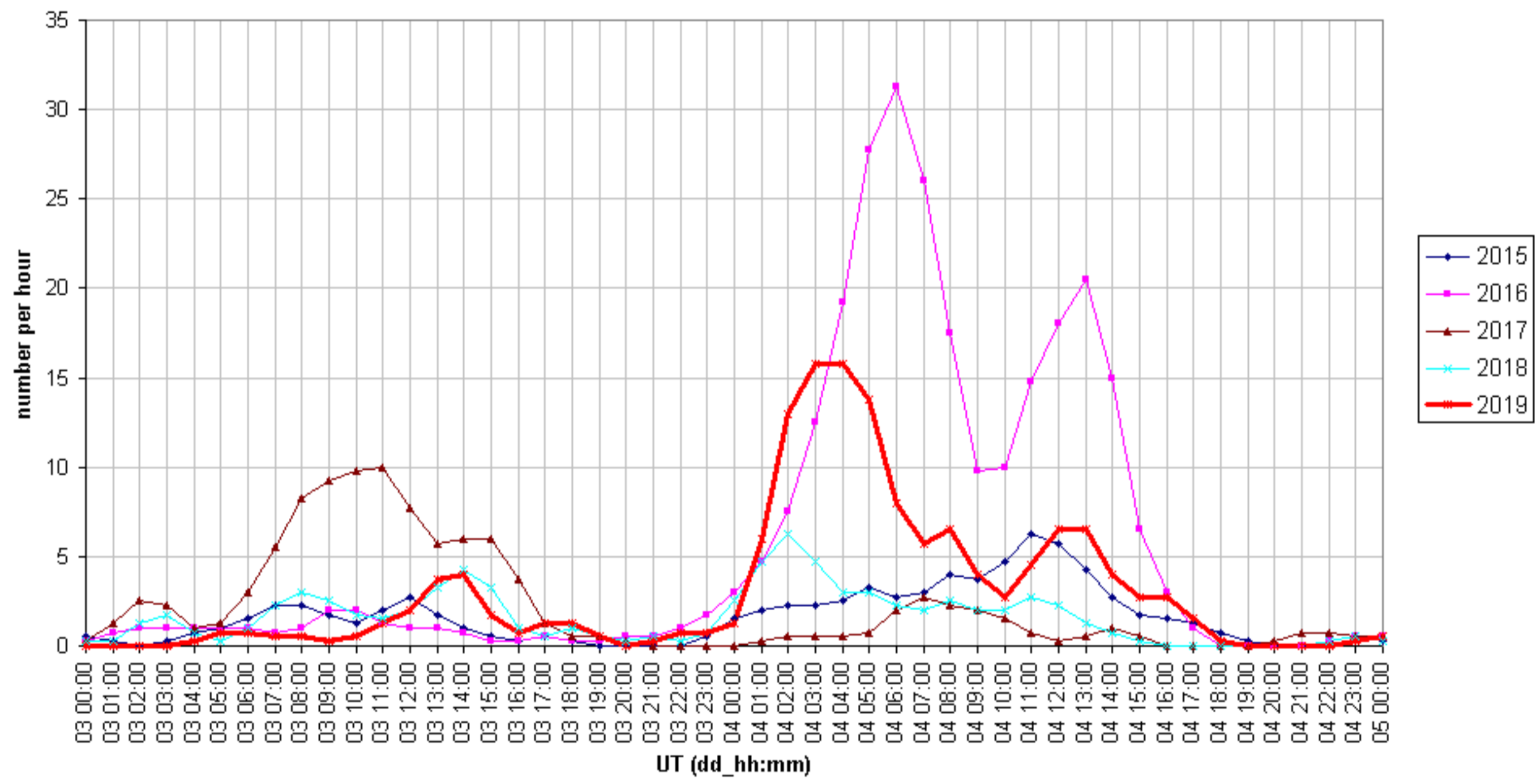
QUA2019_49.99MHz_03+04 January 2019 Overdense reflections longer than 10 seconds (weighted averages) Felix Verbelen (Kampenhout/BE)
