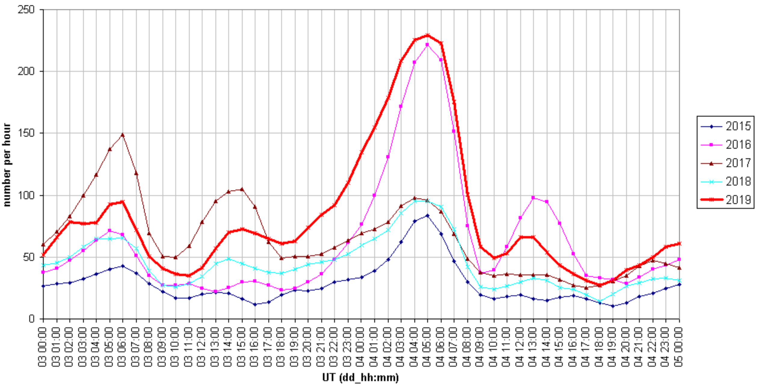
QUA2019_49.99MHz_03+04 January "All" reflections (weighted averages) Felix Verbelen (Kampenhout/BE)
