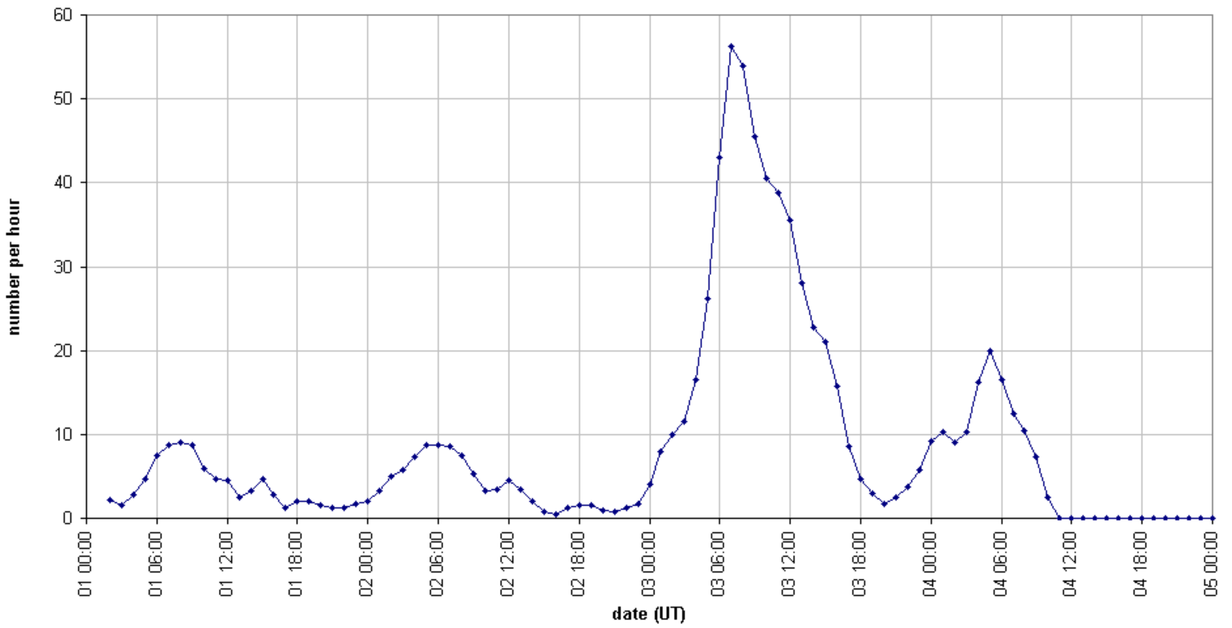
49.99MHz - RadioMeteors January 2017 number of overdense reflections per hour (weighted average) Felix Verbelen (Kampenhout)
