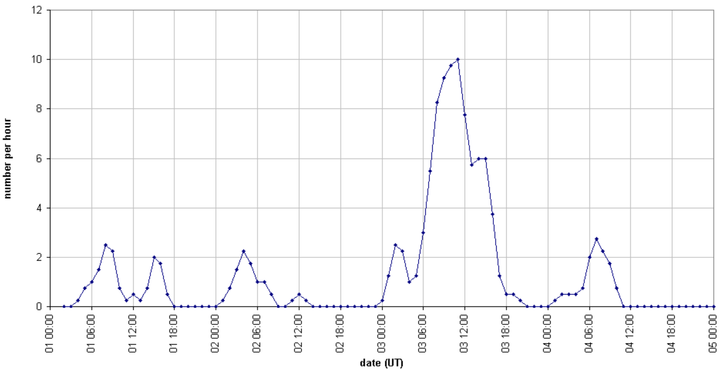
49.99MHz - RadioMeteors January 2017 number of reflections >10 seconds per hour (weighted average) Felix Verbelen (Kampenhout)
