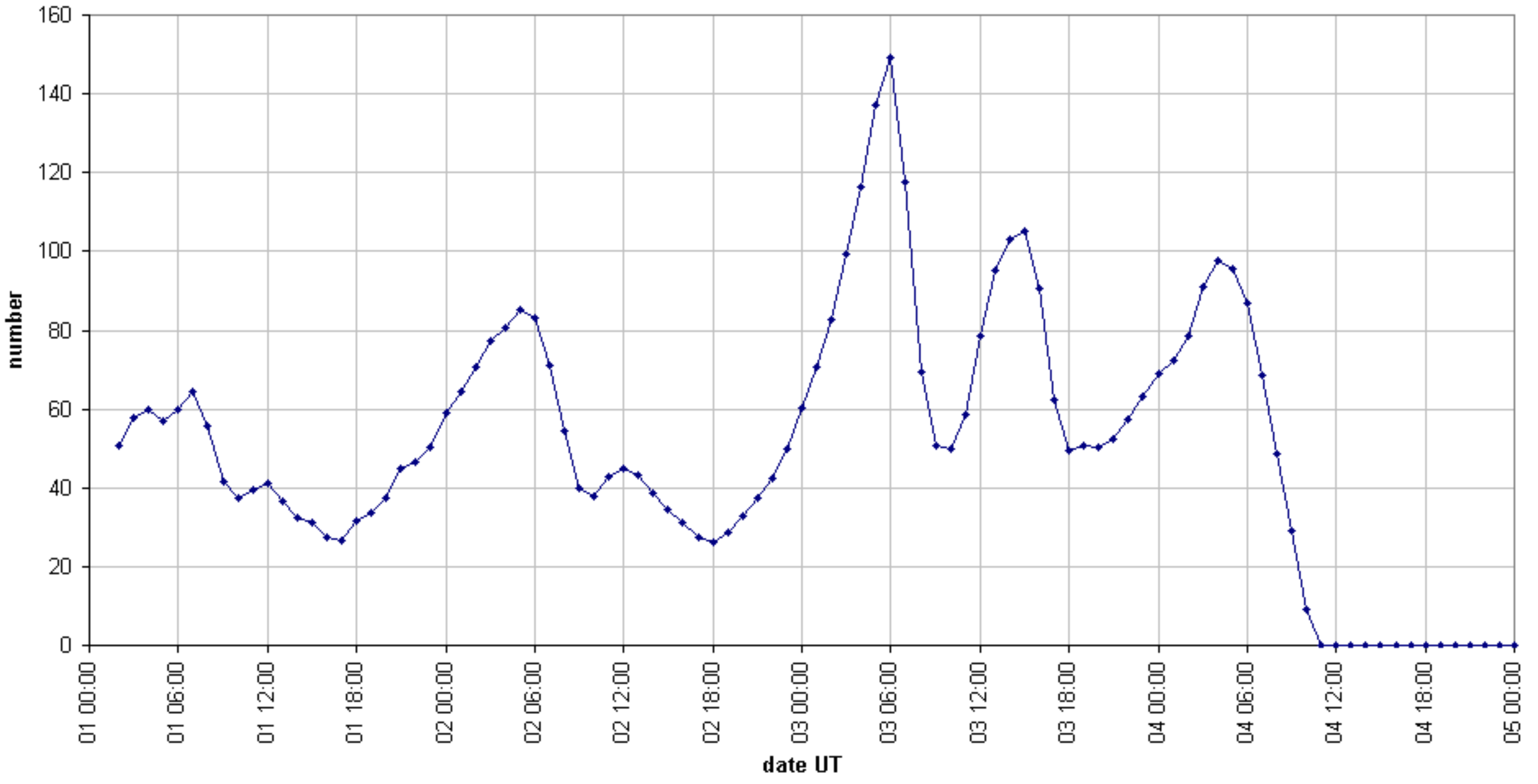
49.99 MHz - RadioMeteors January 2017 number of all reflections per hour (weighted average) (automatic count_MetteI4_7Hz) Felix Verbelen (Kampenhout)
